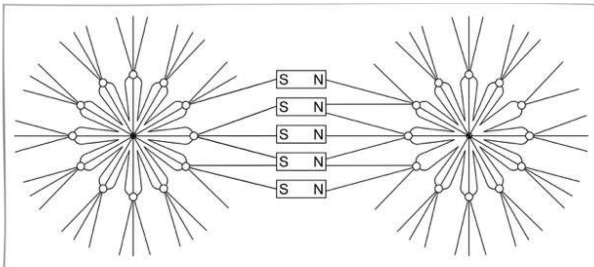
A molecule
