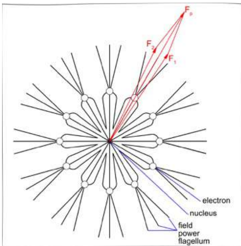
Atom structure – (diameter cross section)
