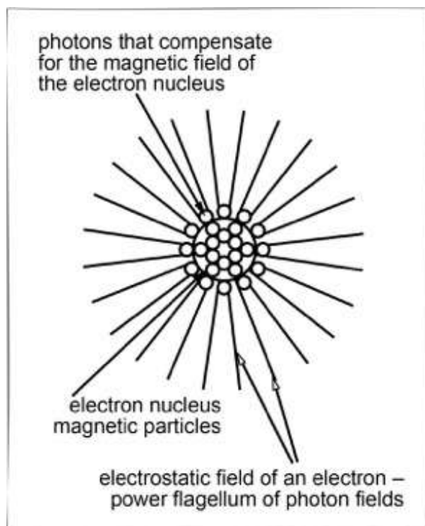
Electron Structure
