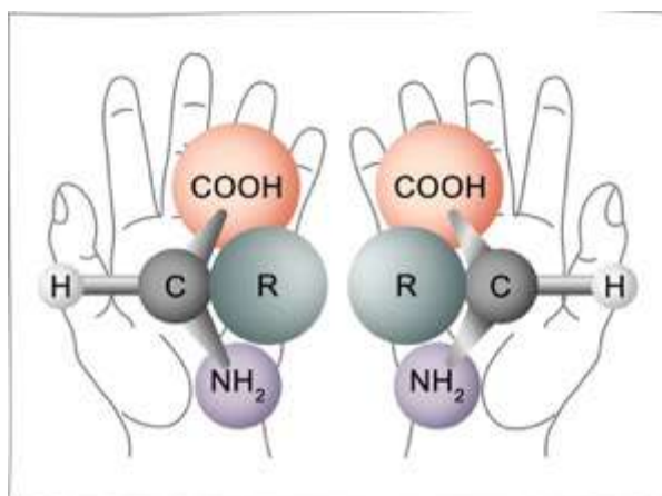
Chirality diagram
