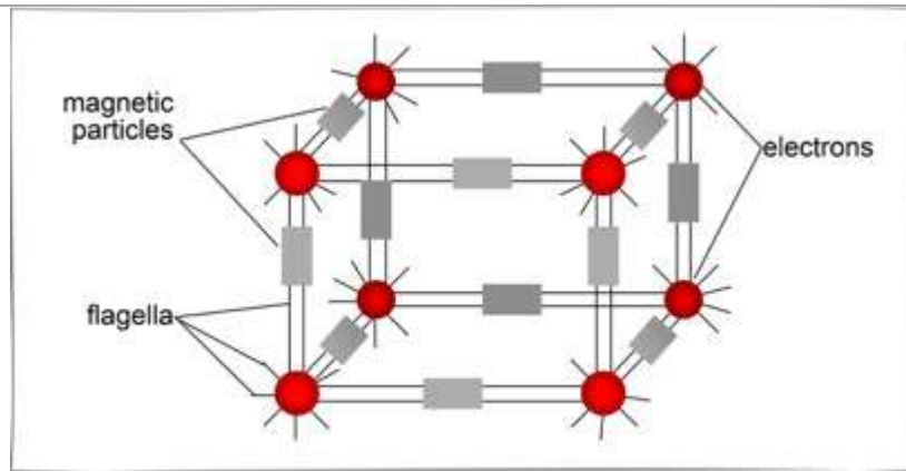
Crystal structure
