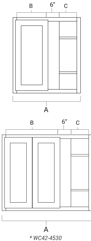
Face Frame Opening Dimensions
