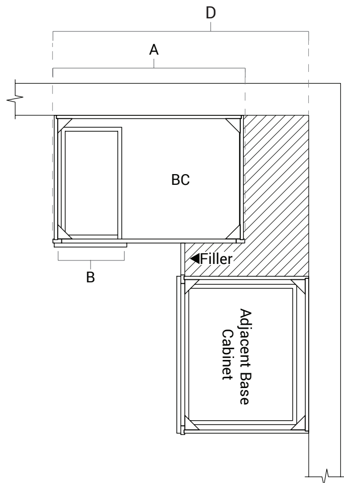
Installation Diagram
