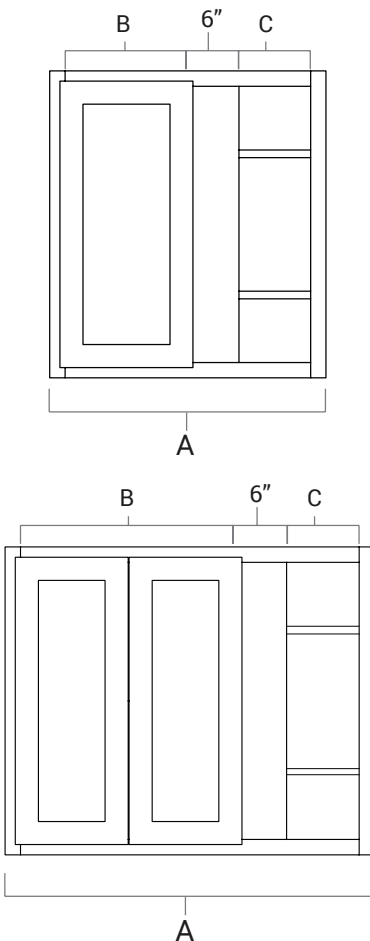
Face Frame Opening Dimensions
