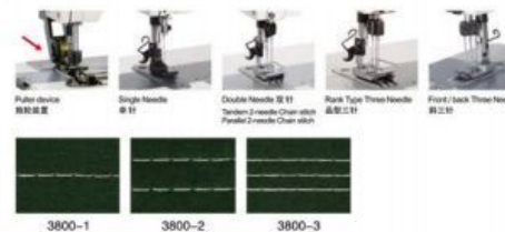
Direct Drive Single/Double needle chainstitch sewing machine with pulter 直驱单/双针链式缝纫机带拖轮
