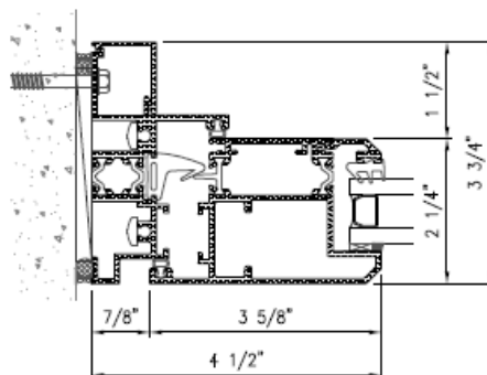
3 LOCK / HINGE STILE
