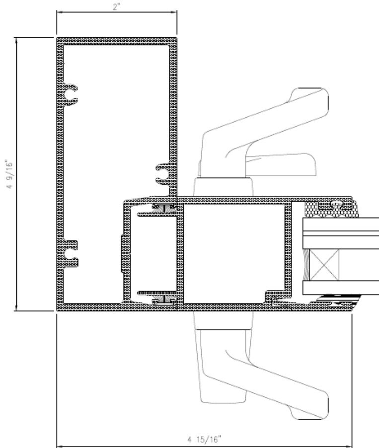
3 MOVING PANEL JAMB
