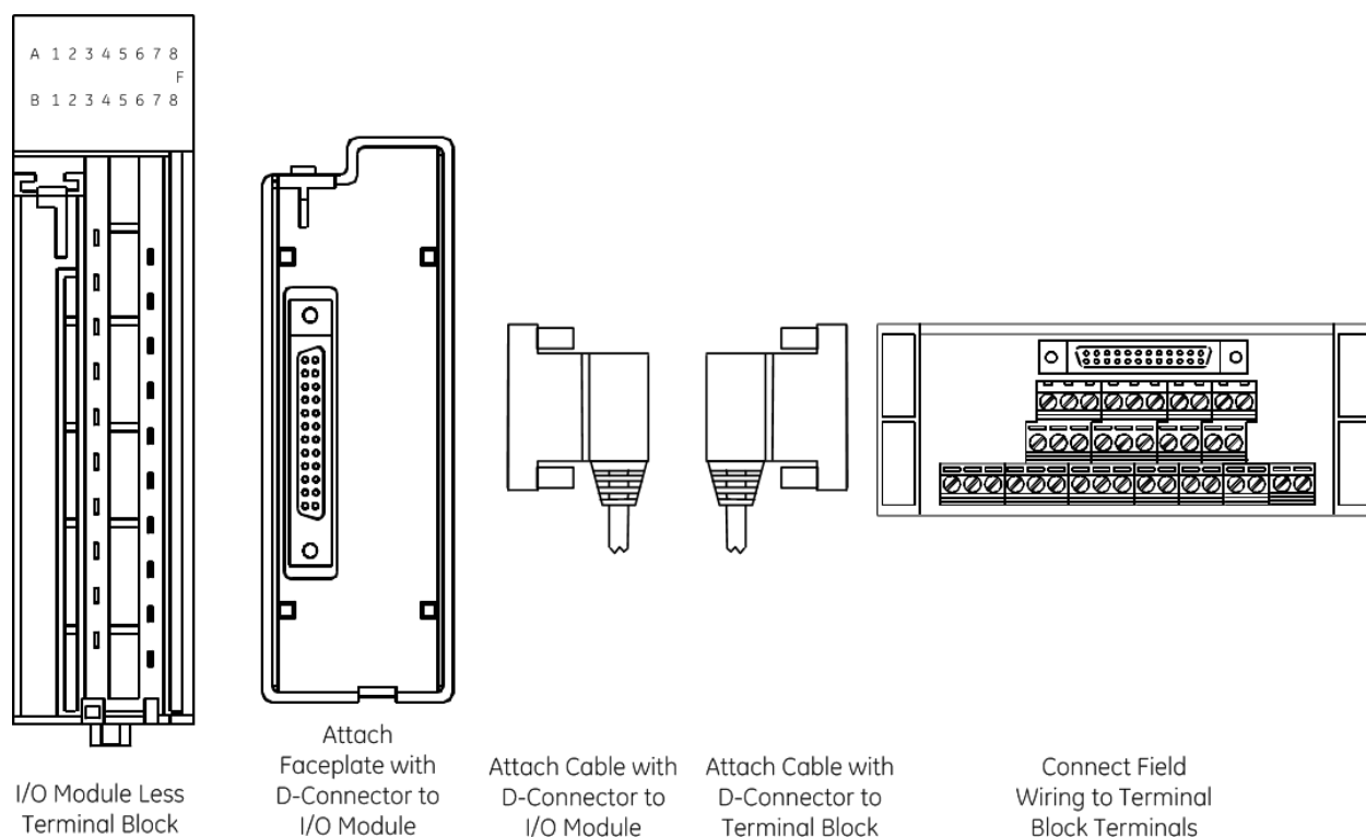
Figure 428: Low-Density Terminal Block Quick Connect System
