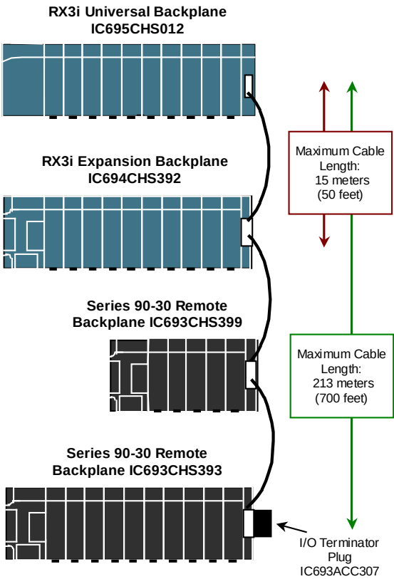
Figure 7: Rx3i System using Expansion and Remote Backplanes
