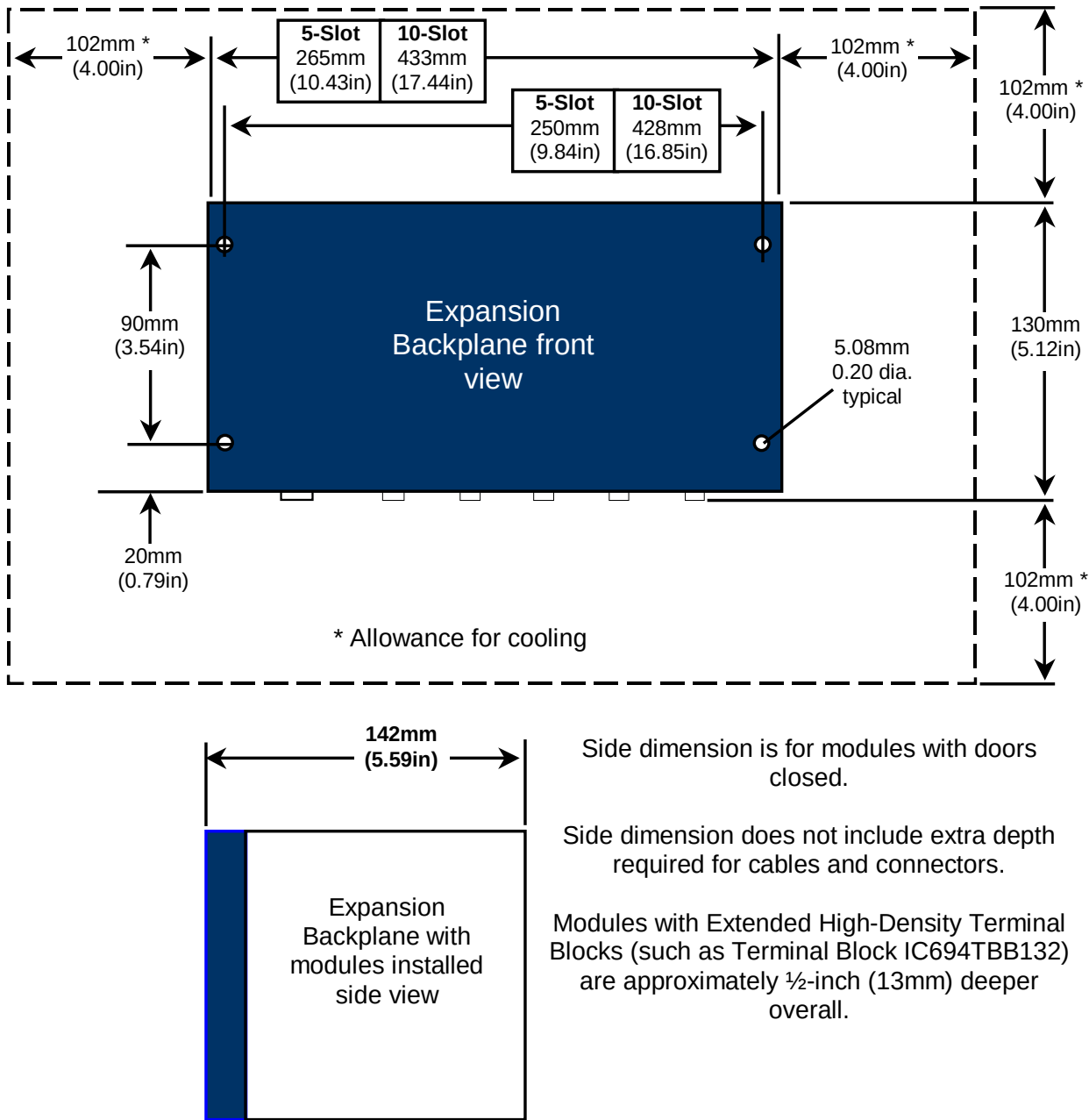
Figure 11: RX3i Serial Expansion Backplane Dimensions and Spacing
