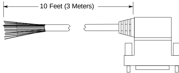
Figure 436: IC693CBL327 and IC693CBL328 Cable Construction
