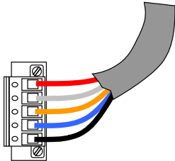
Figure 384: DeviceNet Wiring for End of Segment
