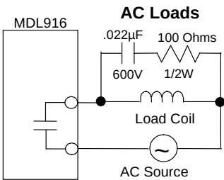
Figure 223: Suppression of AC Loads MDL916
