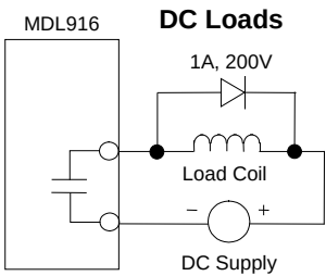
Figure 222: Suppression of DC Loads MDL916
