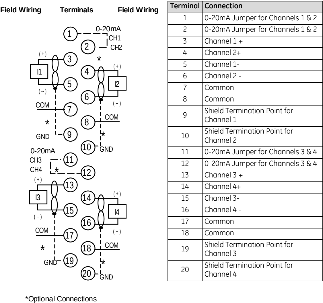
Figure 266: Field Wiring ALG221
