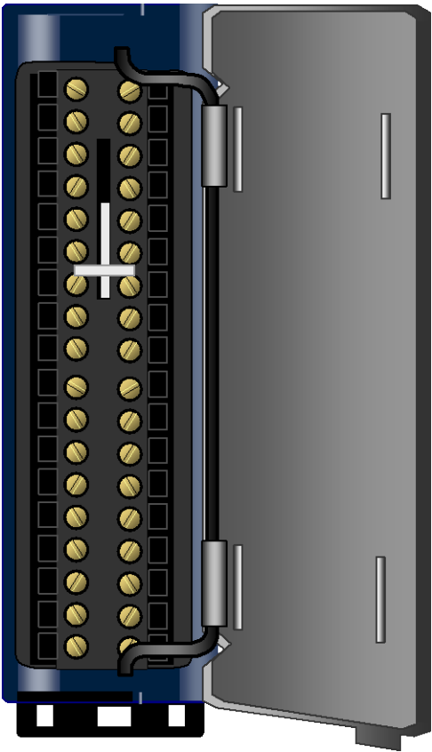
Figure 422: 36-Terminal Box-Style Terminal Block
