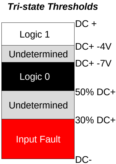
Figure 168: Tri-State Thresholds MDL664
