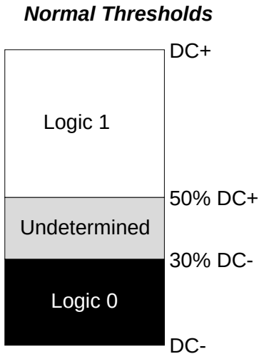
Figure 166: Normal Thresholds MDL664
