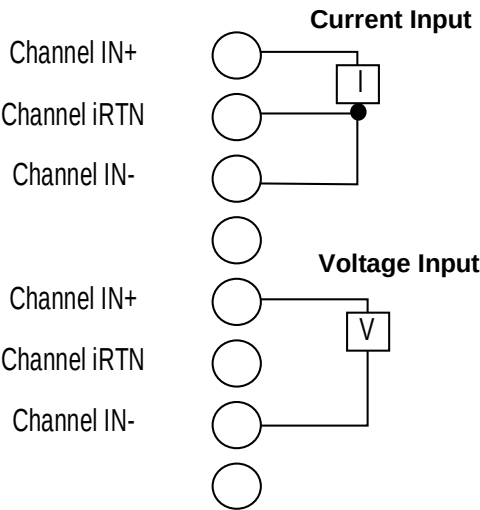
Figure 345: Thermocouple / Voltage / Current Field Wiring ALG600
