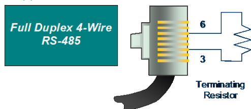
Figure 372: Termination RS-485 4-Wire Full Duplex
