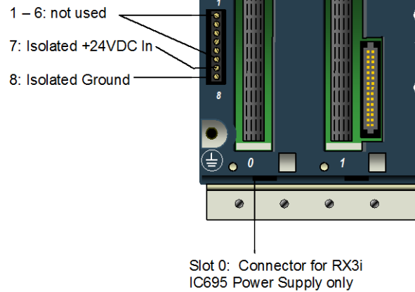
Figure 59: TB1 Terminal Detail
