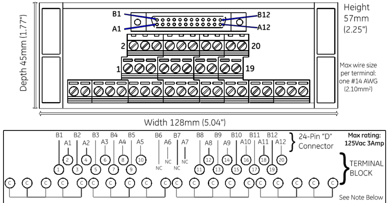
Figure 431: IC693ACC332 TBQC Terminal Block
