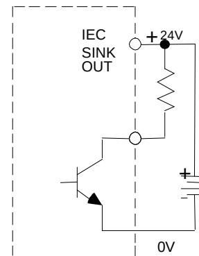
Figure 36: Negative Logic Output Circuit
