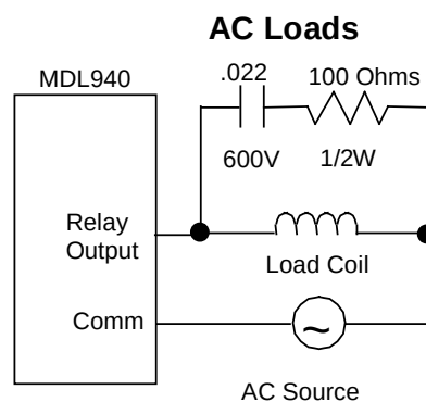
Figure 238: Suppression of AC Loads MDL940
