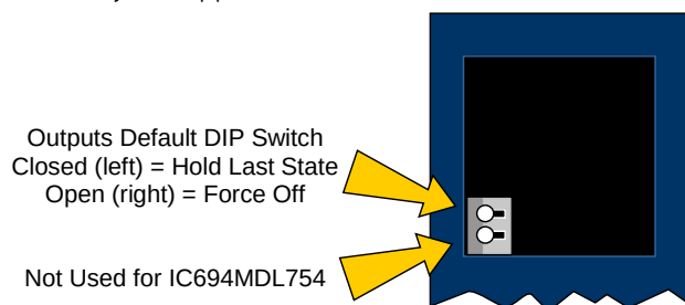
Figure 210: DIP Switch Settings MDL754
