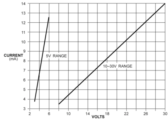
Figure 241: Input Impedance APU300
