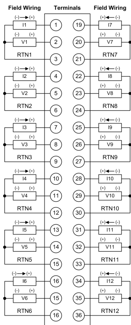
Figure 258: Field Wiring: ALG112
