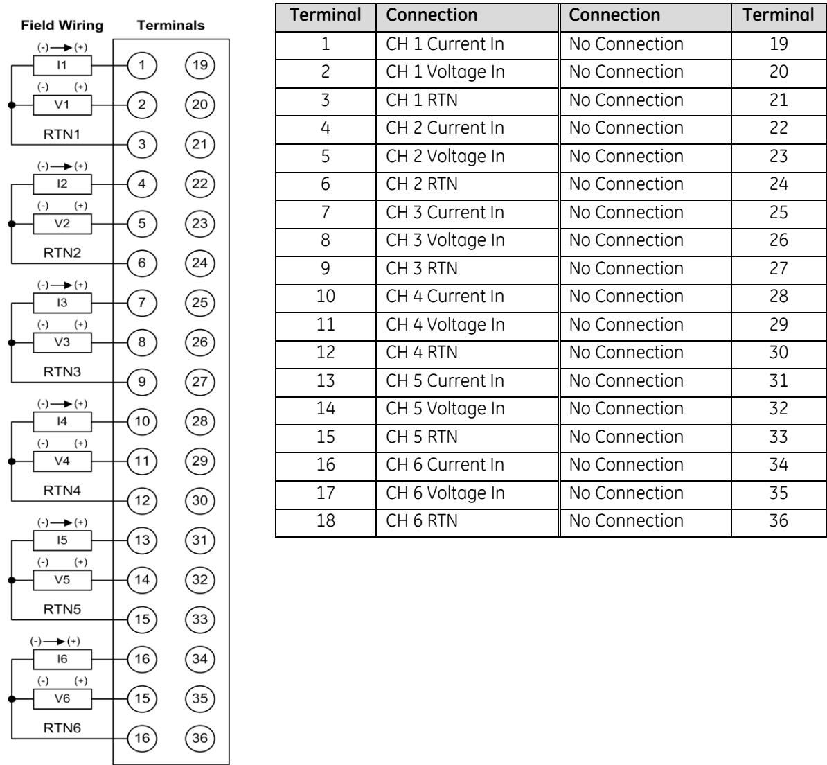
Figure 257: Field Wiring ALG106
