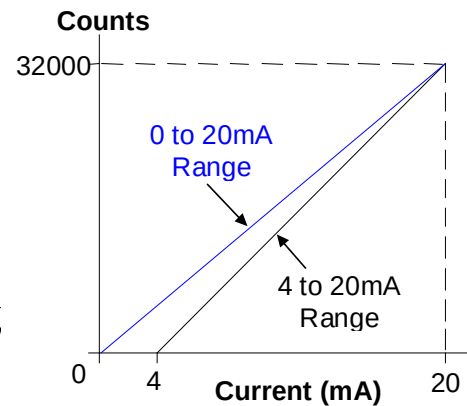
Figure 335: Output Current Scaling ALG442
