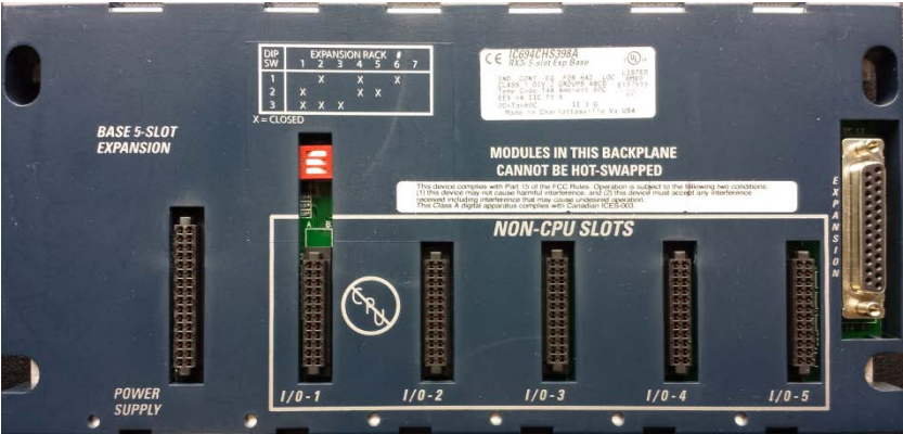
Figure 17: Expansion Backplane
