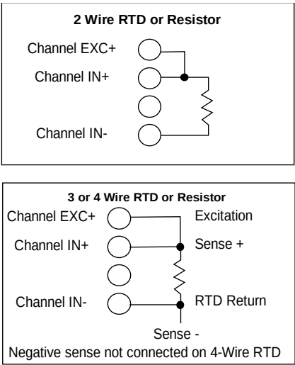
Figure 346: RTD / Resistance Field Wiring ALG600
