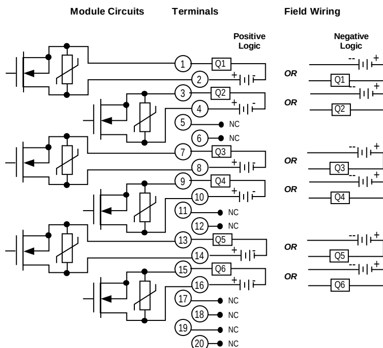
Figure 194: Field Wiring MDL734
