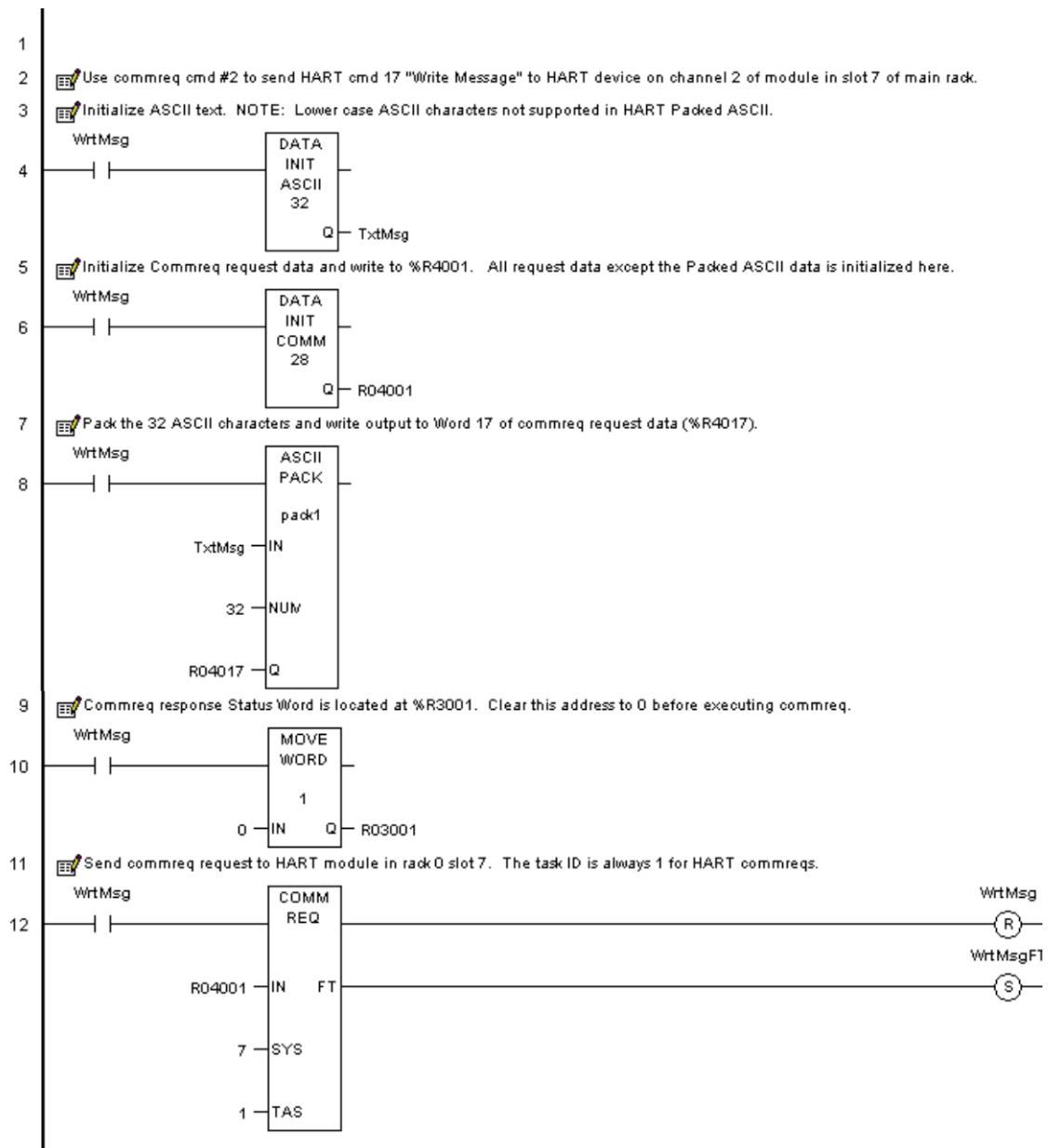
Figure 328: Ladder Logic for ASCII Pack
