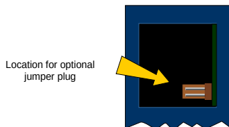
Figure 93: Jumper Location PSA140
