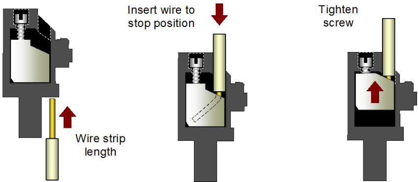
Figure 423: Wire Preparation and Insertion into Box-Style Terminal Block
