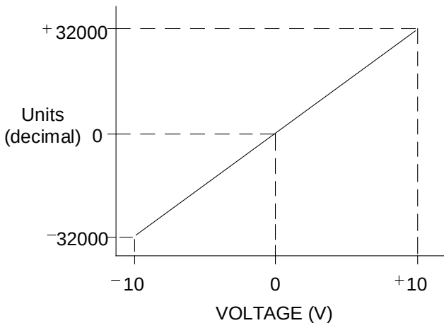
Figure 292: Scaling Units versus Output Voltage
