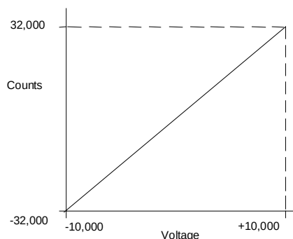
Figure 306: Channel Scaling Example
