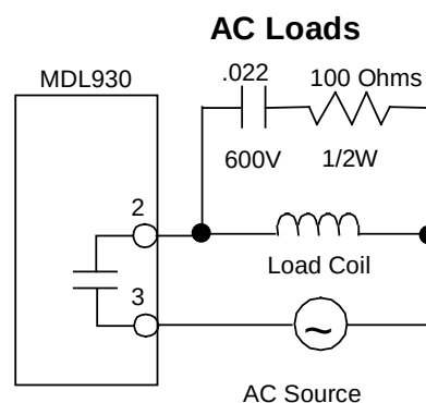
Figure 229: Suppression of AC Loads MDL930
