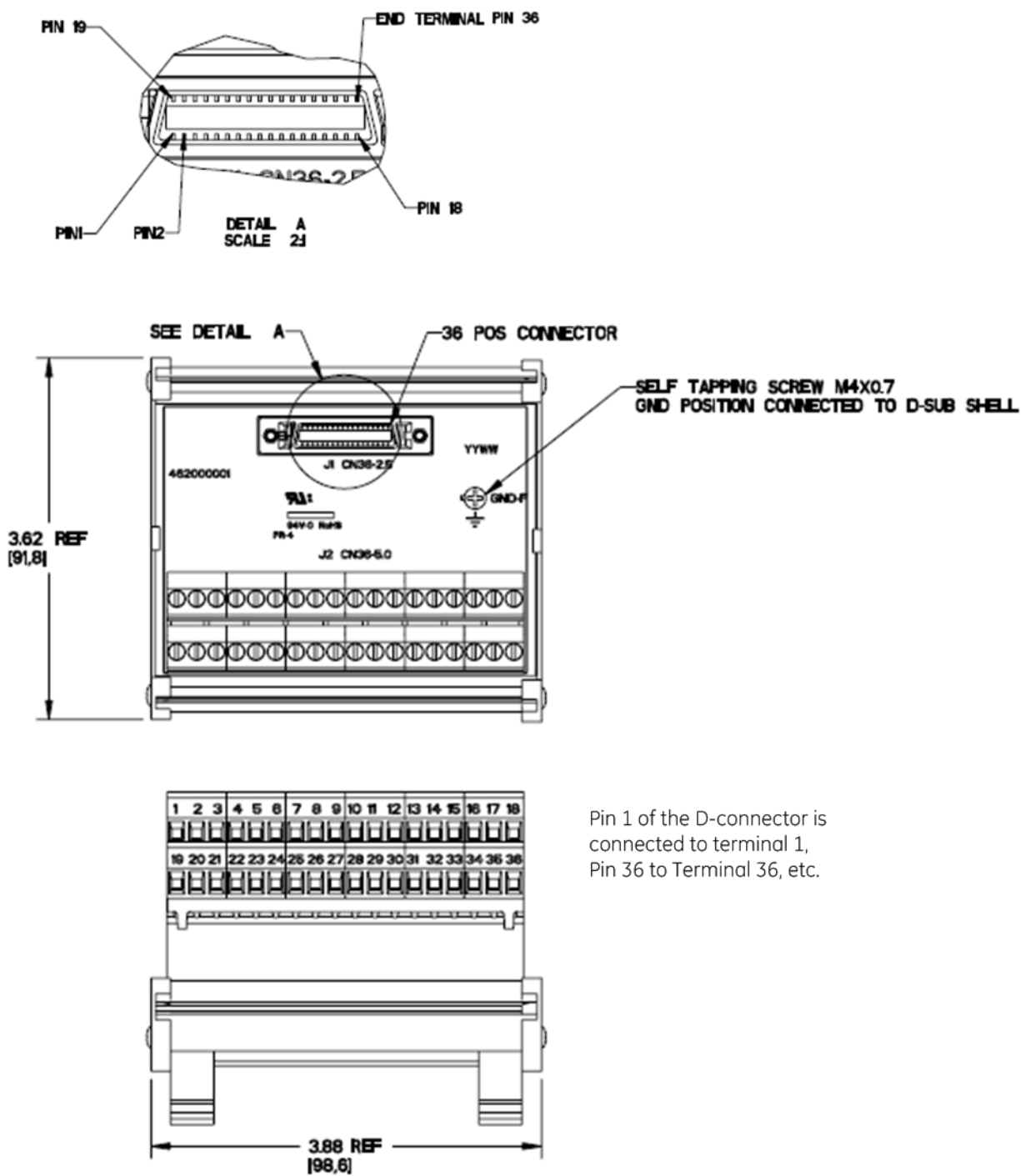
Figure 446: IC694RTB032 High-Density Remote Base, 36-Terminal
