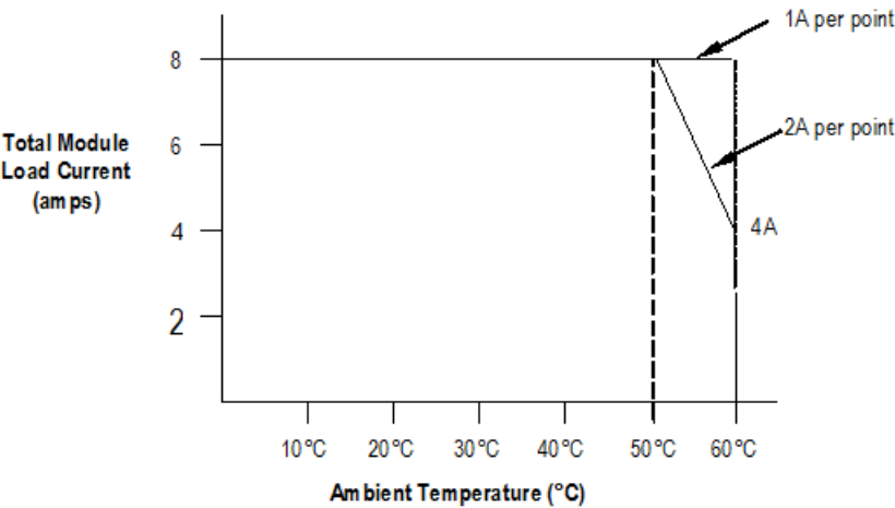
Figure 189: Thermal Derating Curve MDL730
