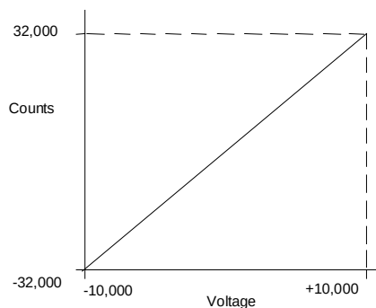
Figure 309: Channel Scaling Example
