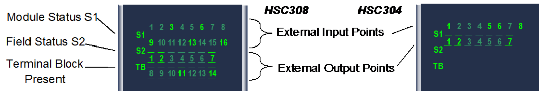
Figure 247: LED Layout HSC304 & HSC308
