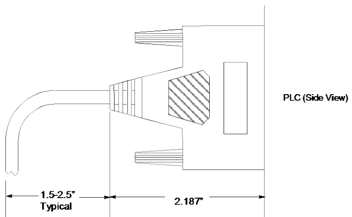
Figure 440: Allowance for Extra Depth using Straight-On Connectors
