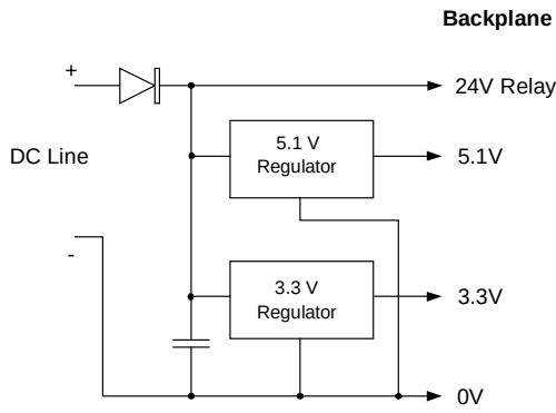
Figure 78: Outputs of Power Supply IC695PSD040 & IC695PSD140
