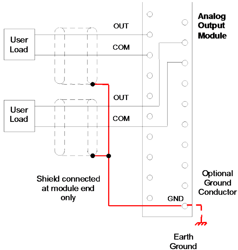
Figure 45: Shield Connections for Analog Output Module
