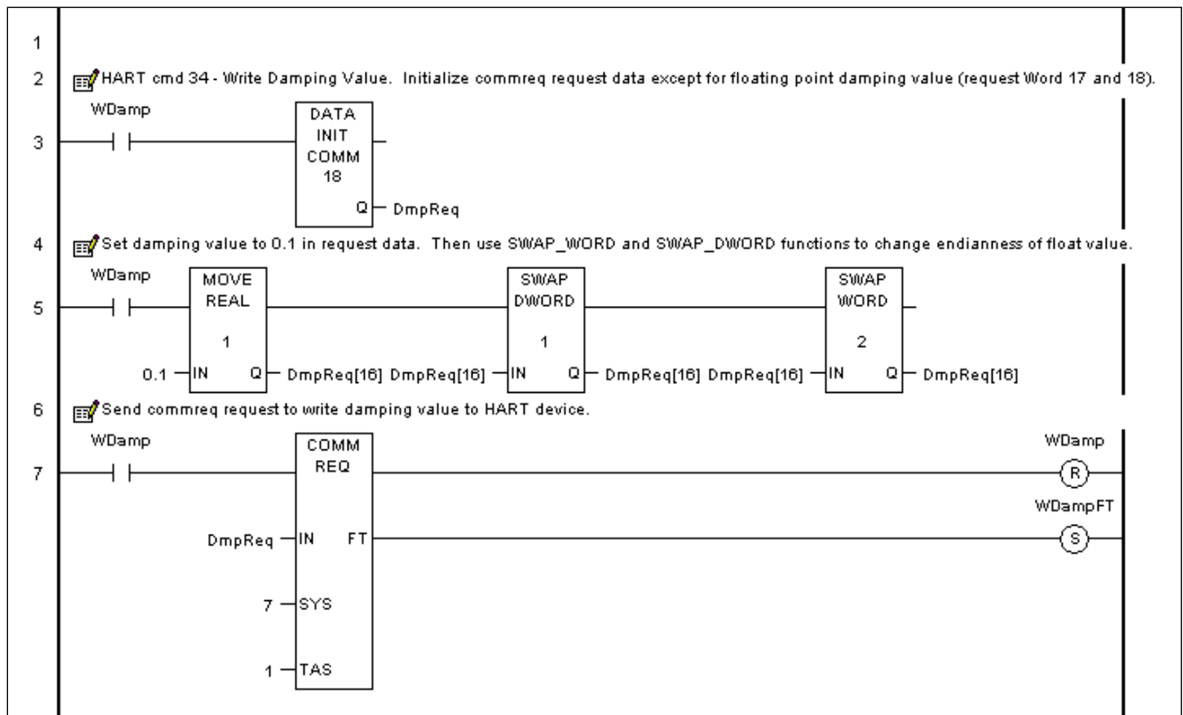
Figure 327: Ladder Logic Using Swap DWord & Swap Word
