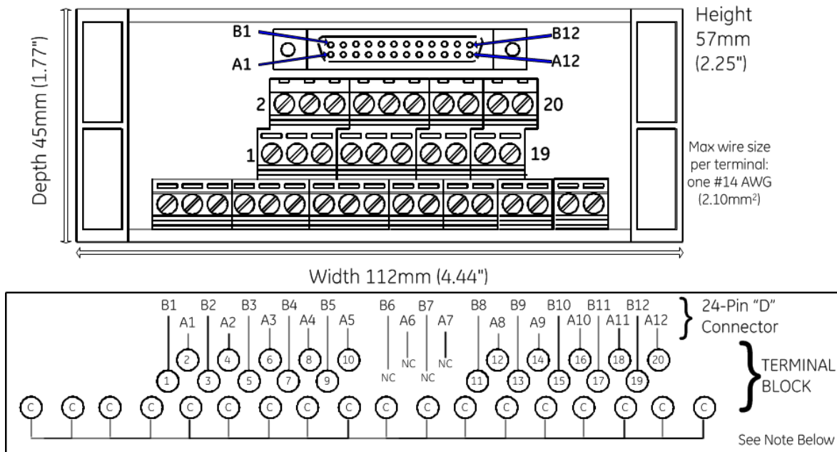
Figure 430: IC693ACC329 TBQC Terminal Block
