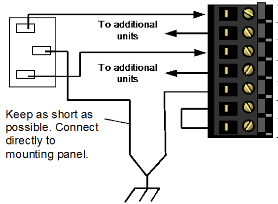
Figure 94: Field Wiring for PSA140
