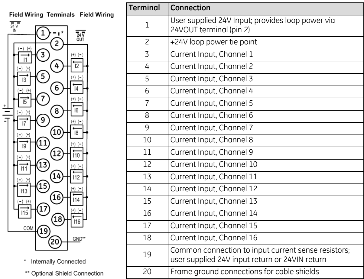
Figure 273: Field Wiring ALG223
