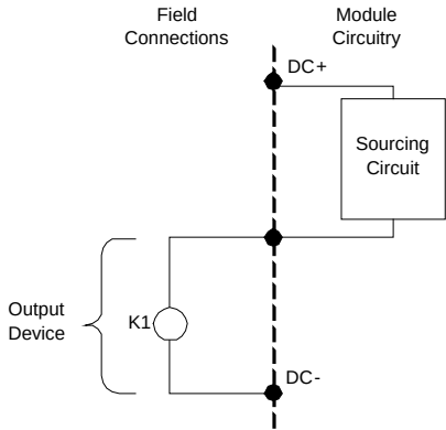
Figure 219: Circuit Detail MDL765
