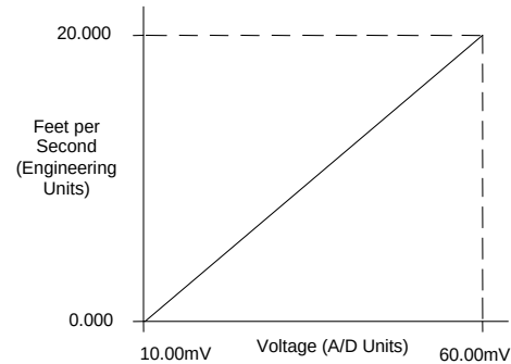
Figure 354: Input Scaling Example 1
