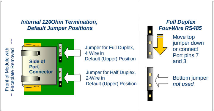
Figure 419: Using the Internal Terminating Resistor PRS015
