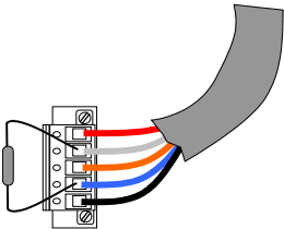
Figure 383: DeviceNet Terminating Resistor Installation
