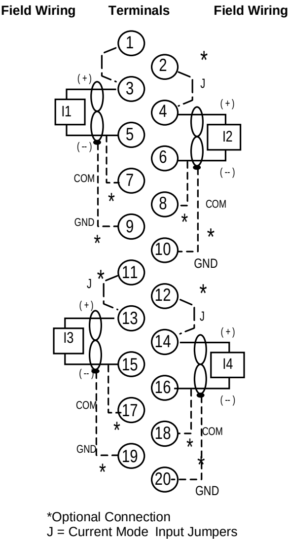
Figure 263: Field Wiring ALG220
