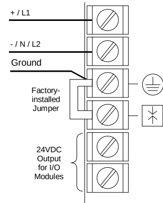
Figure 111: Field Wiring for PWR330
