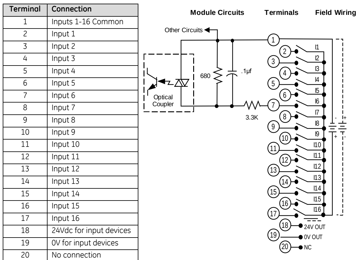
Figure 149: Field Wiring MDL645
