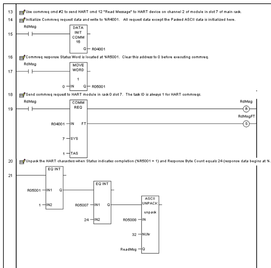
Figure 329: Ladder Logic for ASCII Unpack
