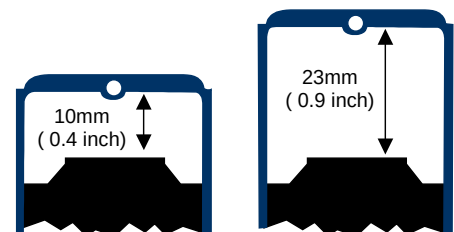
Figure 421: Depth Comparison: High-Density vs Extended High-Density Terminal Block
