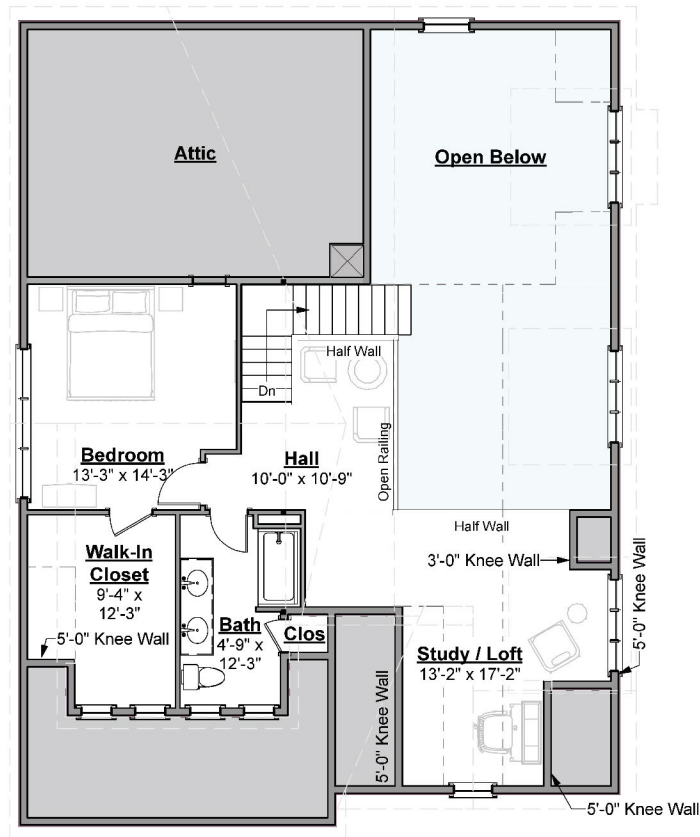
Second Floor - Bedroom / Loft
