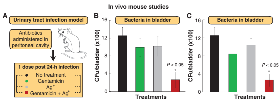
Fig. 6. Ag + potentiates bactericidal anti- biotic activity in vivo in a UTI mouse model.
