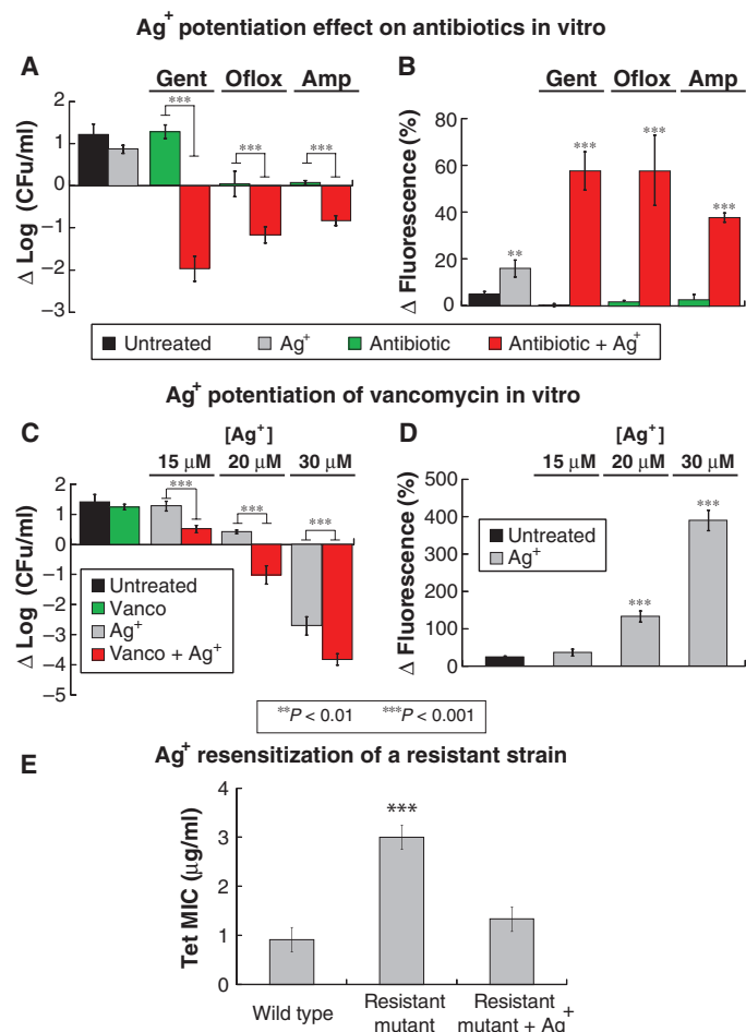
Fig. 3. Ag + potentiates bactericidal antibiotics in vitro. (A) Log change in colony-forming units (CFU)/ml, from time zero, of WT E. coli after treatment for 3 hours with 15 μM AgNO 3 , gentamicin (Gent) (0.25 μg/ml), ofloxacin (Oflox) (0.03 μg/ml), ampicillin (Amp) (1 μg/ml), and combinations of AgNO 3 with the respective antibiotics. (B) Changes in HPF fluorescence after 1 hour of administering the treatments described in (A). (C) Log change in CFU/ml, from time zero, of WT E. coli after treatment for 3 hours with the indicated concentrations of AgNO 3 and vancomycin (30 μg/ml). (D) Changes in PI fluorescence after 1 hour of administering different concentrations of AgNO 3 . Error bars represent means ± SEM from at least six biological replicates. Ten mice per treatment group were used for the survival studies. (E) Treatment of a drug-resistant E. coli strain with Ag + restores antibiotic susceptibility back to WT levels. Tetracycline MIC of WT E. coli (AG110) and that of an E. coli drug-resistant strain (AG112) with and without Ag + treatment. *** P < 0.001 , ** P < 0.05 , Student's t test, significant difference from the WT strain or untreated control, unless otherwise specified. Error bars represent means ± SEM from at least three biological replicates.
