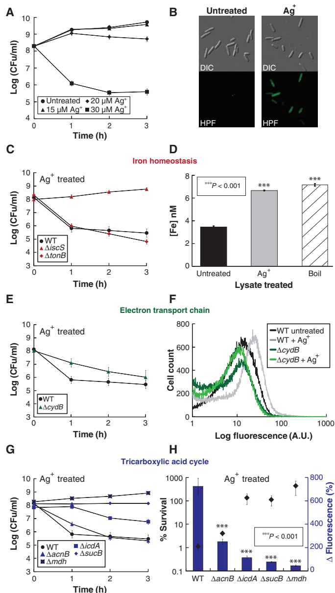
Fig. 1. \text{Ag}^+ induces \text{OH}^\bullet production through a metabolic cascade and iron misregulation. (A) Kill curves for log-phase growing wild-type ( WT ) E. coli treated with various concentrations of \text{AgNO}_3 . (B) Bright-field and fluorescence microscopy of HPF-stained untreated E. coli cells and cells treated with 30 \mu\text{M AgNO}_3 after 1 hour. (C) Survival of iron homeostasis gene knockout mutants relative to WT when treated with 30 \mu\text{M AgNO}_3 . (D) Free iron [ \text{Fe}^{2+} ] concentration in a cell lysate after 1 hour of treatment with heat (90°C) or 30 \mu\text{M AgNO}_3 . (E) Survival of an electron transport gene knockout mutant relative to WT when treated with 30 \mu\text{M AgNO}_3 . (F) GFP fluorescence histogram from the soxS reporter, incorporated into a WT and \Delta\text{cydB} strain of E. coli , after 1 hour of treatment with 30 \mu\text{M AgNO}_3 . (G) Survival of tricarboxylic acid (TCA) cycle gene knockout mutants relative to WT when treated with 30 \mu\text{M AgNO}_3 . (H) Blue bars show percent change in fluorescence for HPF (hydroxyl radical production), HPF-stained WT, and TCA cycle mutant strains of E. coli treated for 1 hour with 30 \mu\text{M AgNO}_3 relative to the HPF-stained untreated strains. The diamond data points represent percent survival after 1 hour of treatment with 30 \mu\text{M AgNO}_3 . Error bars represent means \pm SEM from at least three biological replicates. *** P < 0.001 , Student's t test, significant difference from the untreated lysate in (D) and the treated WT in (H).
