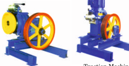
Traction Machine
