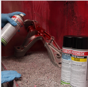
LIQUID PENETRANT
