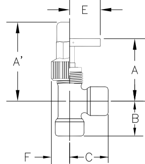
FPT X FPT, ANGLE
