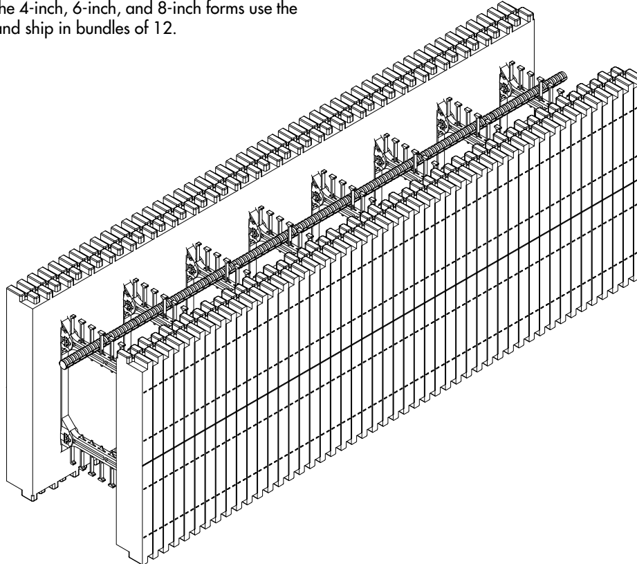
Figure 1.2.1 BuildLock BL-800 Assembled Straight Block. This block fully integrates with all other BuildBlock products. The web bridges are fully reversible inside the block for additional rebar placement options.
