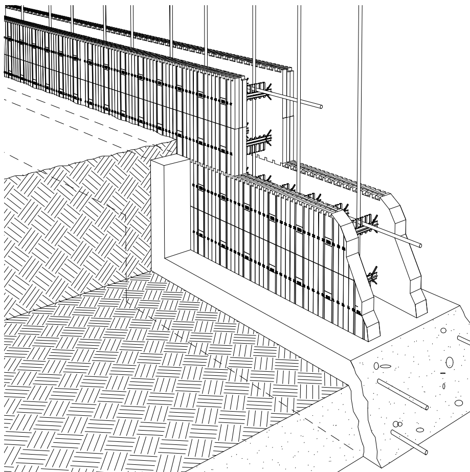
Figure 4.3.4 Step footing transition using full height blocks. Built-in half-height blocks may also be used for smaller transitions, putting the cut side down.
