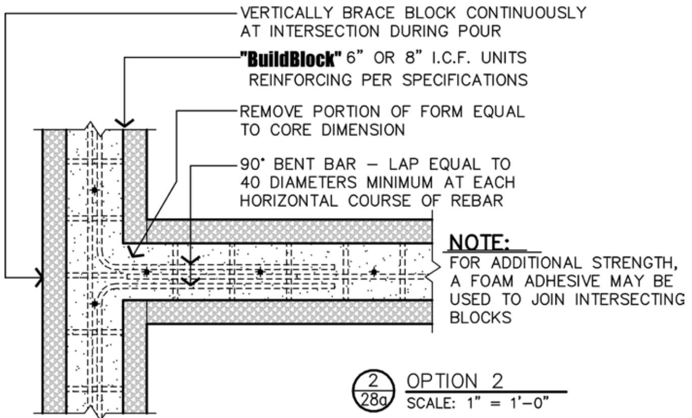
Figure 5.5.10 Intersecting wall construction details.
