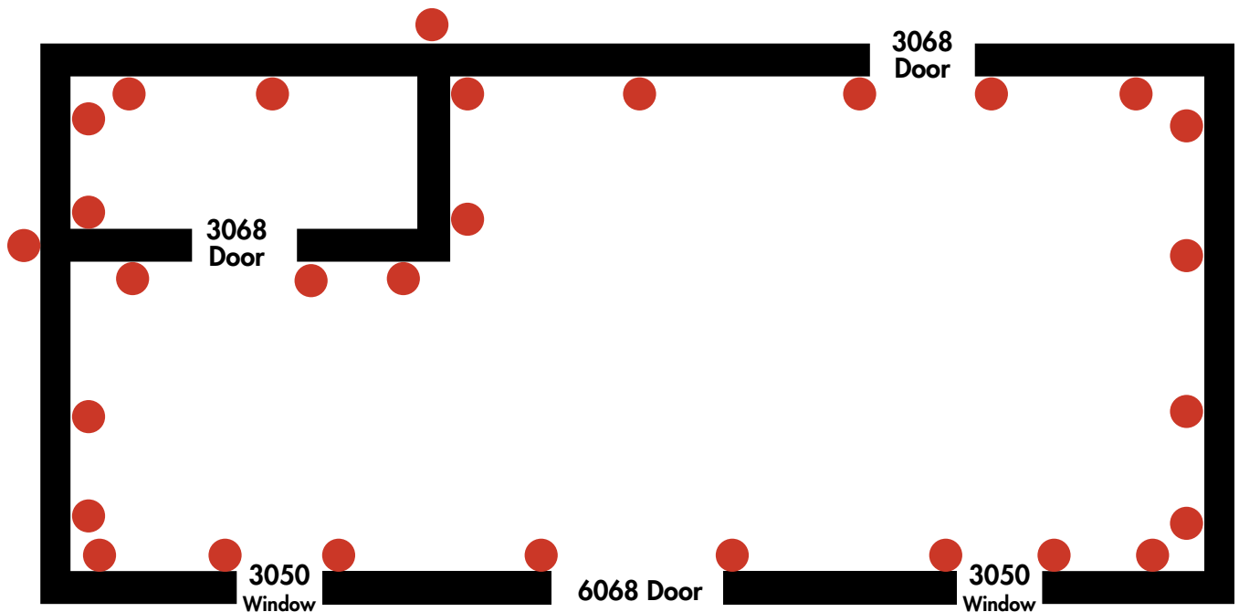
Figure 9.5.2 Example interior wall bracing. The red dots indicate a recommended location for a brace.
