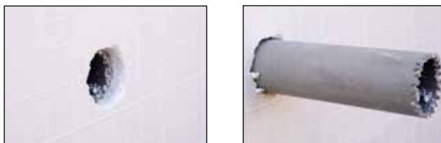
Figure 7.1.3 Cut small teeth on one end of the pipe sleeve and use to saw through the other side of the block to create a smooth opening.
