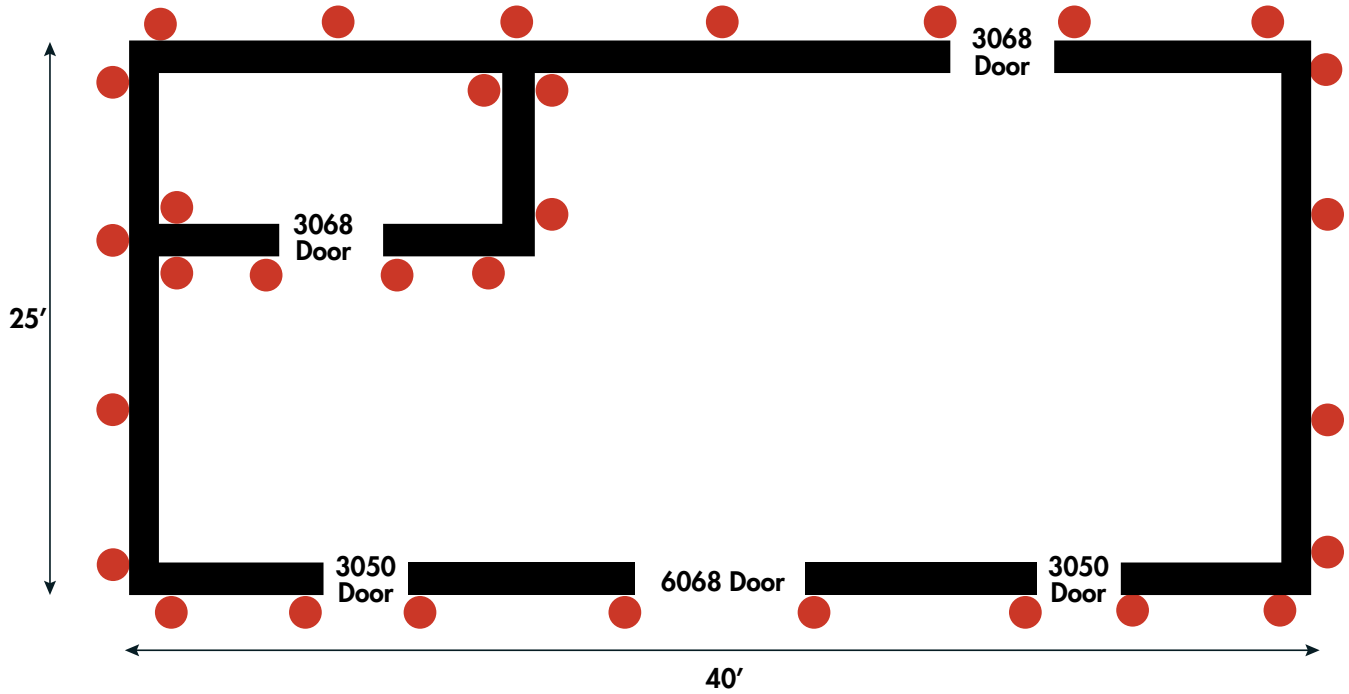
Figure 9.5.1 Example exterior wall bracing. The red dots indicate a recommended location for a brace.
