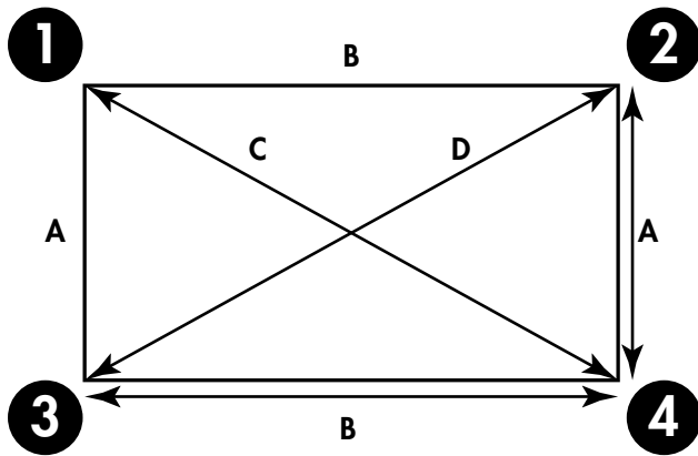
Figure 4.1.3 Diagonal Squaring Method
