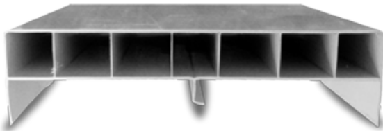
Figure 8.1.3 Section of V-Buck Vinyl Bucking. When assembling seal exposed holes with spray foam to prevent concrete from filling the buck and creating a thermal bridge.
