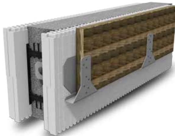
Figure 5.10.3 Steel bearing plate embedded into the top of an ICF wall. Ensure the correct height taking into account the interlock.
