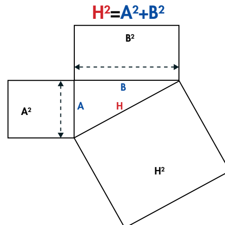
Figure 4.1.2 Pythagorean Theorem (3-4-5) Method.
