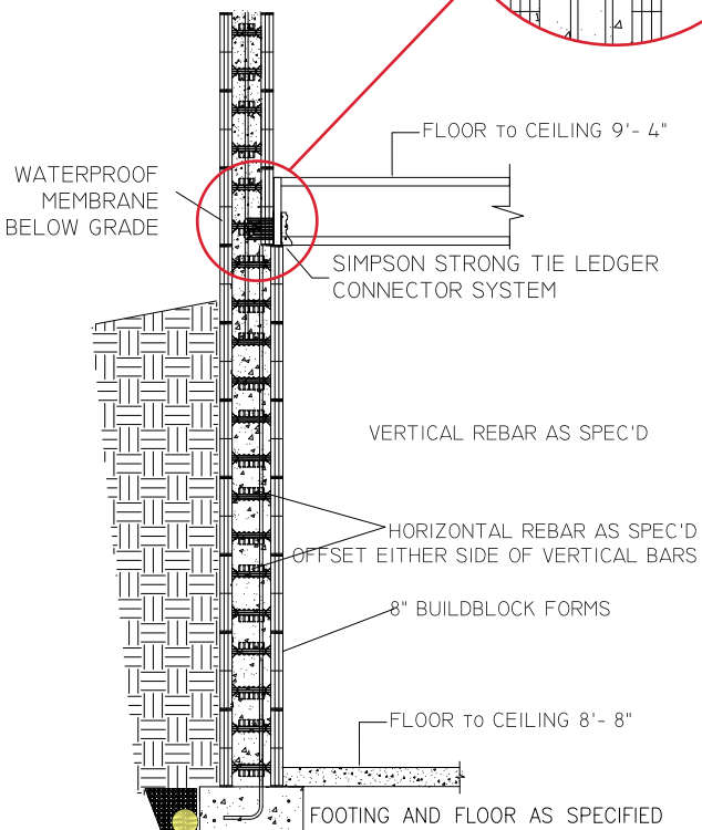
TYPICAL 8" BUILDBLOCK BASEMENT WITH 6" BUILDBLOCK ABOVE. GABLE CROSS SECTION
