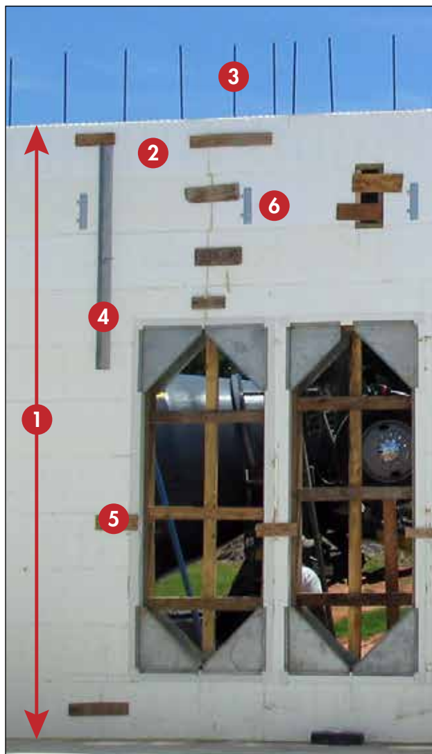
Figure 5.8.2 Second story construction example.
