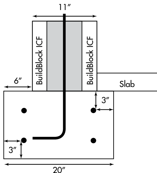
ICF Footing Example using BuildBlock BB-600 6" forms. ACI 318 requires all rebar in concrete touching soil have at least 3-inches of concrete cover.
