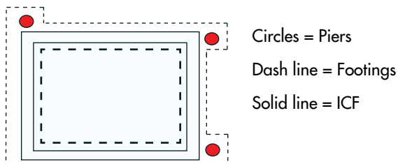
Figure 6.4.8 Basement ICF, Concrete Pier, and Footing design.
