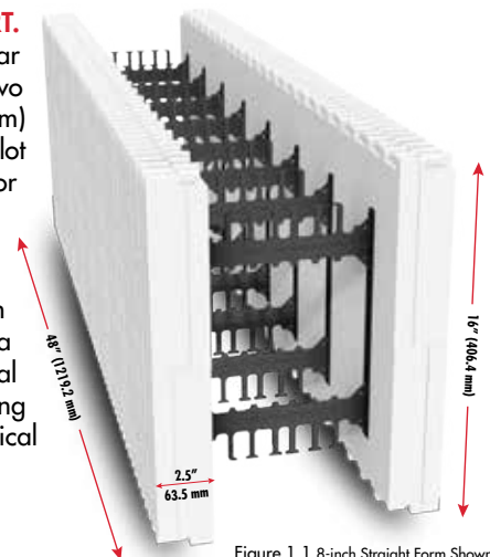
Figure 1.1 8-inch Straight Form Shown
