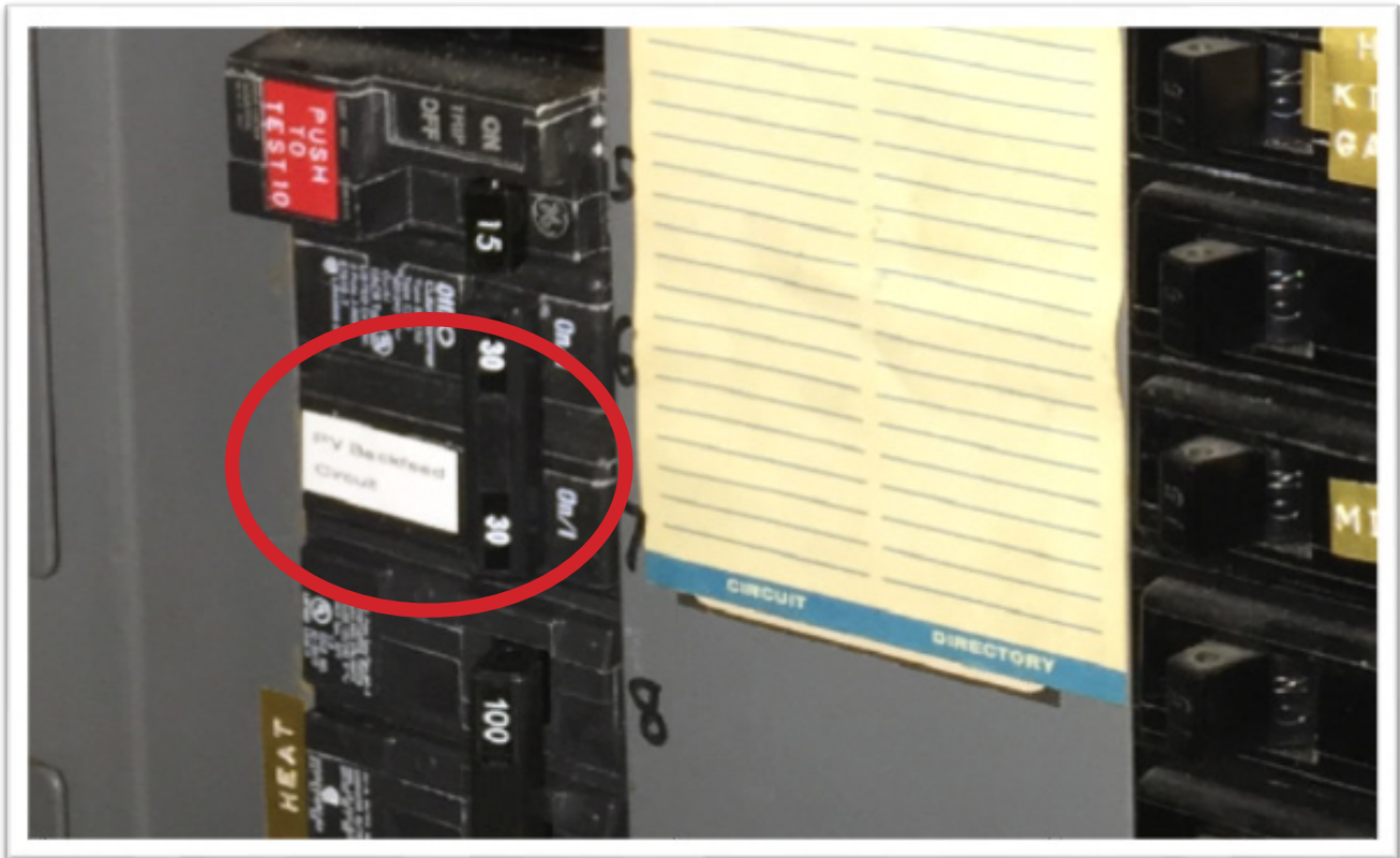
Photo D2: Backfed PV breaker not installed at opposite end of buss bar from main breaker: 2014 NEC690.12(D)(2)(3)(b)
