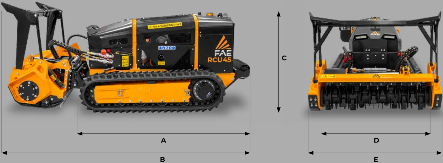
A Overall lenght without attachment B Transport lenght with BLO/RCU attachment on ground
