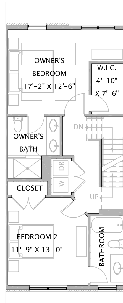
THIRD FLOOR
