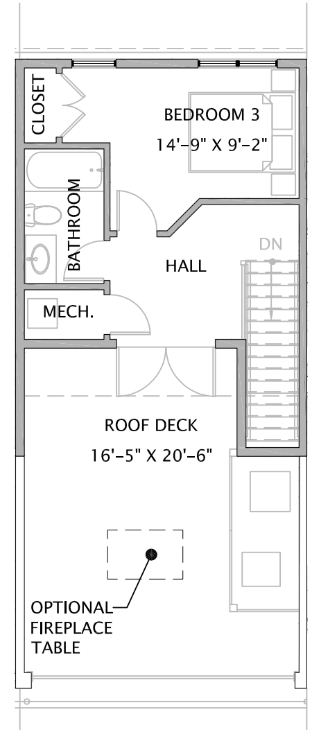
FOURTH FLOOR
