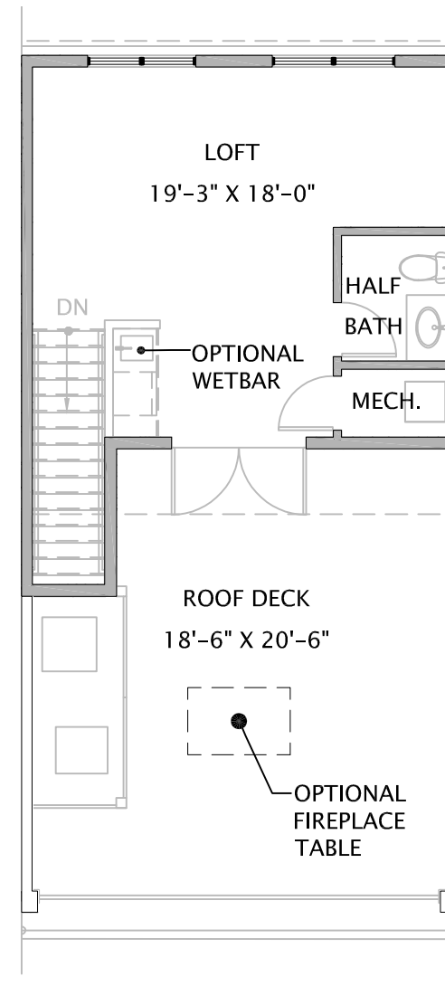
ALTERNATE FOURTH FLOOR
