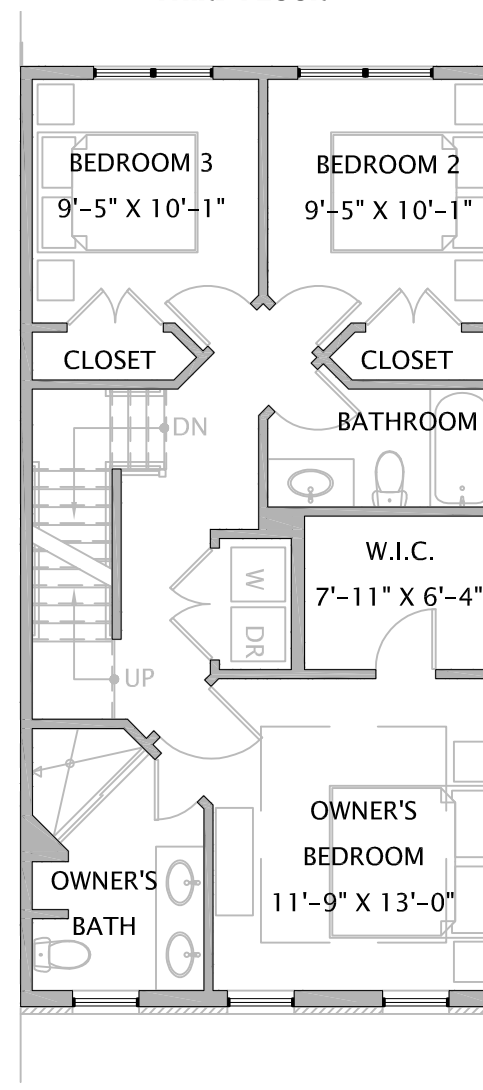
ALTERNATE THIRD FLOOR
