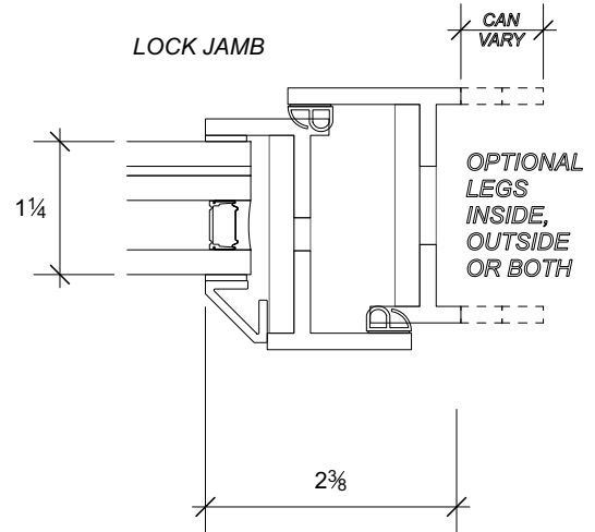
FS-56i 3000 OUT-SWING WINDOW FS-56i 5000 OUT-SWING DOOR
