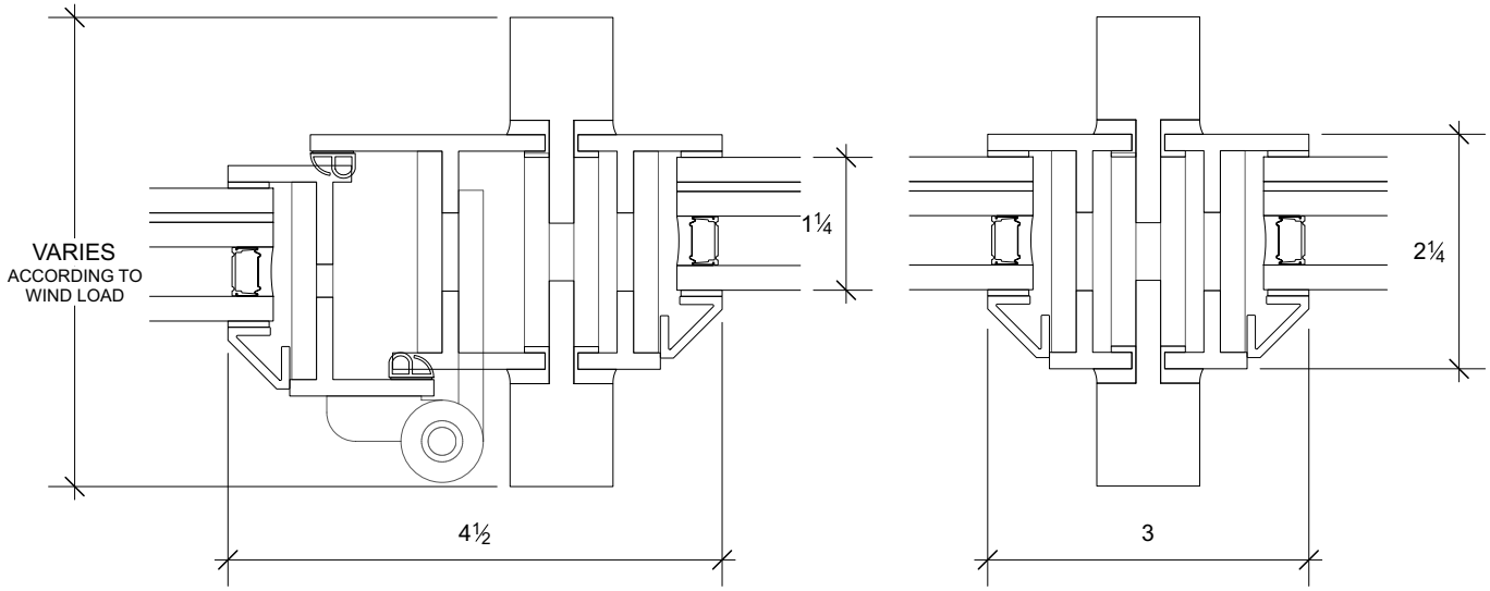
OPERABLE TO FIXED
