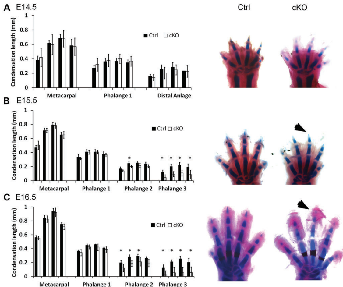
Figure 2. Atrx ( Prx1 ) cKO digit defects appear at embryonic day 15.5. (A) Phalange length measurements from embryonic day 14.5 Atrx fl/yPrx1cre (CTRL) and Atrx ( Prx1 ) cKO (KO) mice. No differences are seen in the length of cartilaginous condensations in the forelimb. (B) Phalange length measurements at embryonic day 15.5. cKO mice exhibit shortening of terminal phalanges. (C) Phalange length measurements from embryonic day 16.6. All distal phalanges are significantly shortened in mutant mice. * P < 0.05, n = 3.
