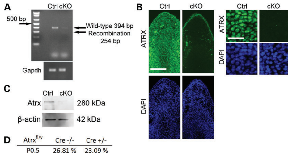
Figure 1. Atrx is deleted in the forelimbs of Atrx (Prx1) cKO mice. (A) RT-PCR analysis of RNA isolated from embryonic forelimbs of Atrx fl/y Prx1 cre males Atrx (Prx1) cKO (KO) and control littermates (Ctrl). Amplification was performed with primers flanking the loxP sites, in introns 17 and 20. Recombined RNA in Atrx (Prx1) cKO is unstable and degraded. (B) Cryosections of E15.5 forelimb tissue were stained for ATRX protein. Atrx (Prx1) cKO mice lack ATRX in the nucleus of all mesenchyme tissues. Scale bar: 200 \mu m (representational high-resolution image: 50 \mu m) (C) Immunoblot of proteins isolated from E15.5 forelimbs shows loss of ATRX protein in Atrx (Prx1) cKO mice. (D) Atrx (Prx1) cKO mice are born at normal Mendelian ratios, with no associated lethality.
