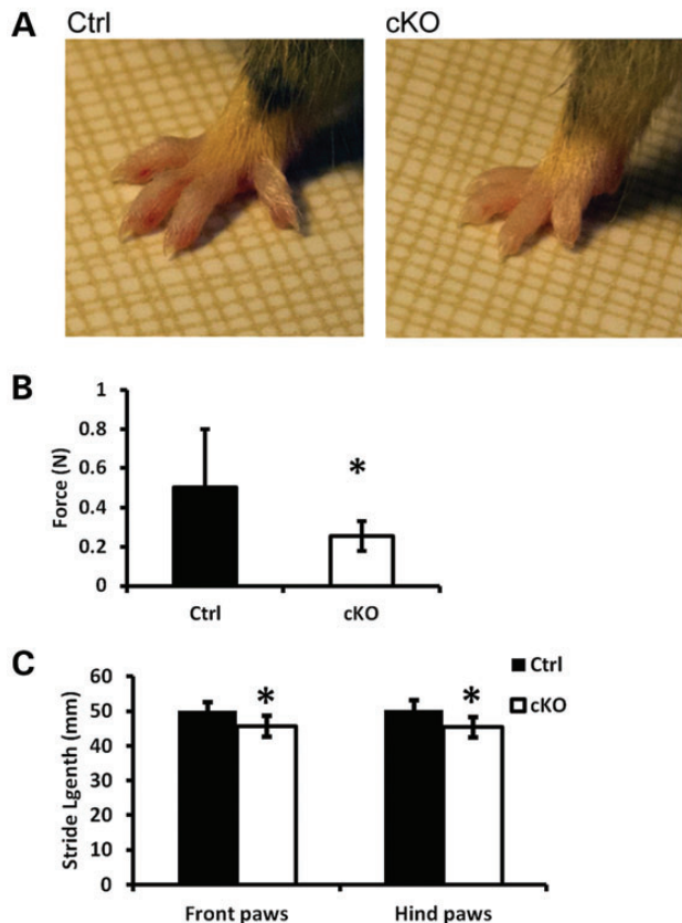
Figure 7. Reduced forelimb function at 1 year of age in Atrx ( Prx1 ) cKO mice. (A) Characteristic forelimb appearance of Ctrl and Atrx ( Prx1 ) cKO mice showing shortened fingers and a smaller paw. (B) Forelimb grip strength of control and mutant adult mice. Mutant mice exert significantly less force with their forelimbs before releasing the bar. (C) Quantification of mouse gait parameters. Stride length of the fore- and hind-paws is shorter in Atrx ( Prx1 ) cKO mice.
