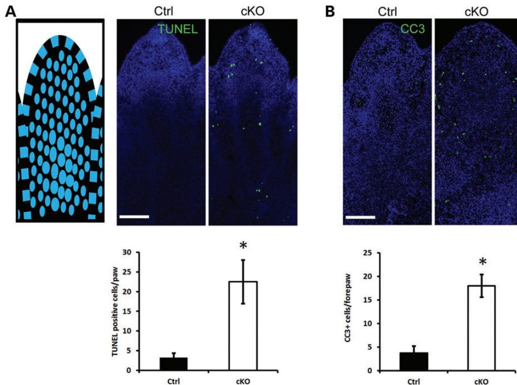
Figure 5. Cell death is increased in the Atrx ( Prx1 ) cKO embryonic limb bud. Fluorescent TUNEL and activated caspase 3 stains of frozen sections for embryonic day 13.5 forelimbs. (A) At E13.5, more TUNEL positive nuclei are observed per digit tip in mutant forelimb sections ( n = 4 ). (B) Atrx ( Prx1 ) cKO embryonic limb buds contain significantly more cells containing activated caspase 3. Scale bar: 200 \mu m error bars = SEM.
