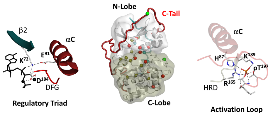
FIG 2 Structure of the PKA catalytic subunit. The first protein kinase structure of the PKA C-subunit, highlighted in the middle panel, revealed the conserved protein kinase fold and provided a three-dimensional framework for the subdomains that were defined previously by the sequence alignments (24). The C-terminal tail is shown in red, the N-lobe is in white, and the C-lobe is in tan; red dots indicate the conserved residues identified by sequence alignment. On the left is the conserved regulatory triad that was predicted to be in close proximity to the phosphates of ATP. On the right is the phosphorylated activation segment showing how this phosphate, pThr197, nucleates many of the subdomains and motifs described in Fig. 1.
