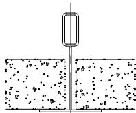
15/16" Flat Ceiling
