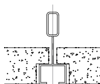
9/16" Slot Ceiling
