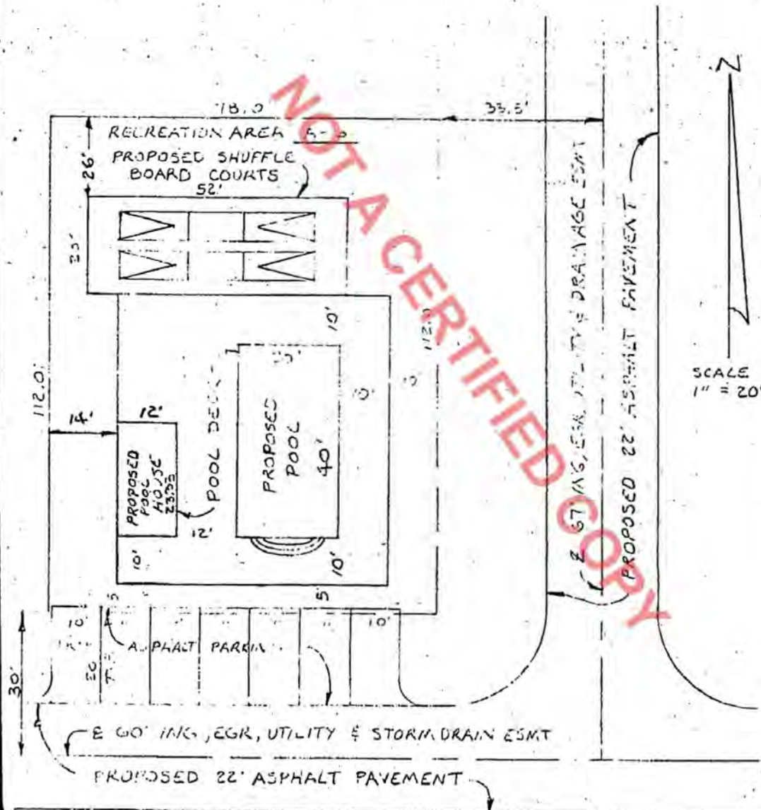
SITE PLAN, RECREATION AREA A-6
