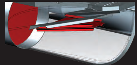
Aluminum Lateral Nose Cone Reinforcement
