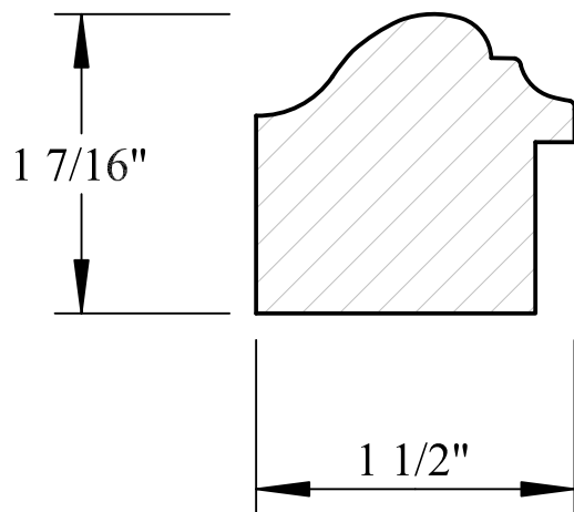
K0-551 B
