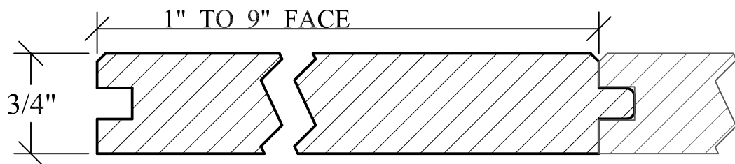
N0-021 (Micro-Vee)
