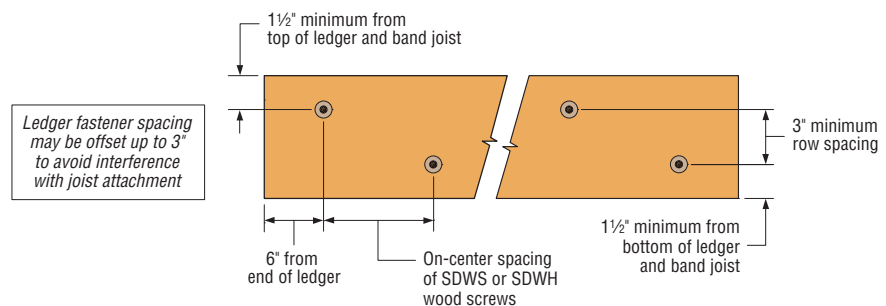
SDWS/SDWH Screw Spacing Detail
