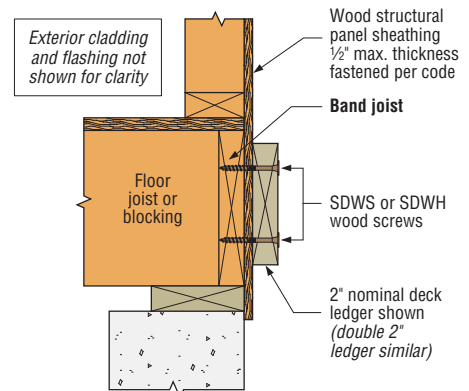
Ledger-to-Band Joist Assembly
