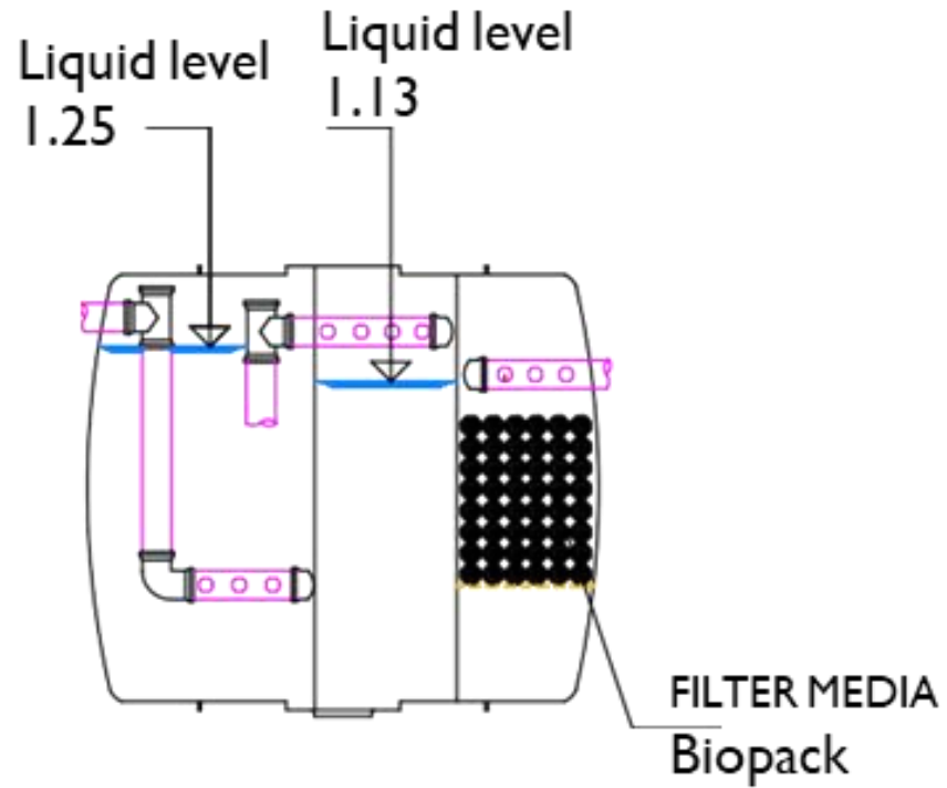
Sectional View Internal - Fillings
