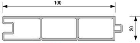
100x20 Panel Profili P.A.099.5400
