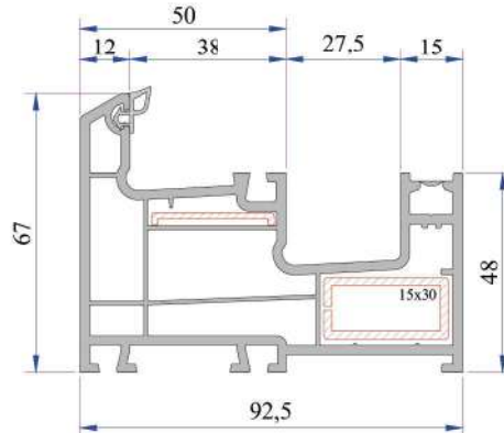
Tek Ray Kasa P.A.232.1105.650.0.BC.01
