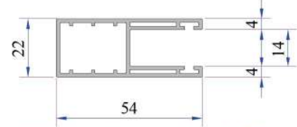
155x155mm Panjur Yan Ray Profili P.A.097.5609.600.0.00.19
