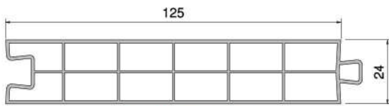
125x24 Panel Profili P.A.099.5408
