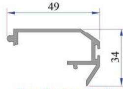
Alm. Kapama Profili 16013.601.5.2.0.0000
