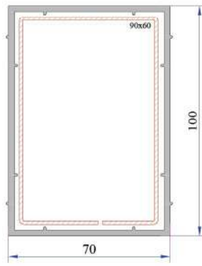
70x100 mm Kutu Profili P.A.070.5202.600.0.00.19
