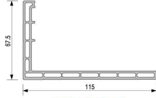
Pervaz Profili (67,5x115) P.A.099.5505
