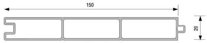
Panel Profili P.A.099.5407
