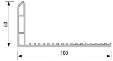
Pervaz Profili (50x100) P.A.099.5501
