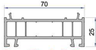
Frame Lifting Profile 25 mm P.A.070.5306.600.0.00.19
