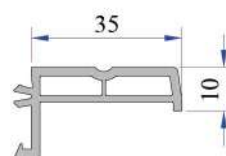
Kasa Pervaz Profili (35mm) 099.5523
