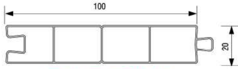
100x20 Yeni Panel Profili P.A.099.5401
