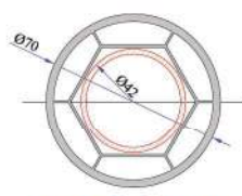
Ø70 Boru Profili P.A.070.5106.600.0.00.19
