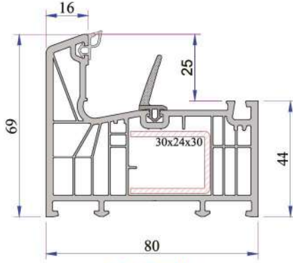
Kasa Profili P.A.888.1000.600.2.BC.01
