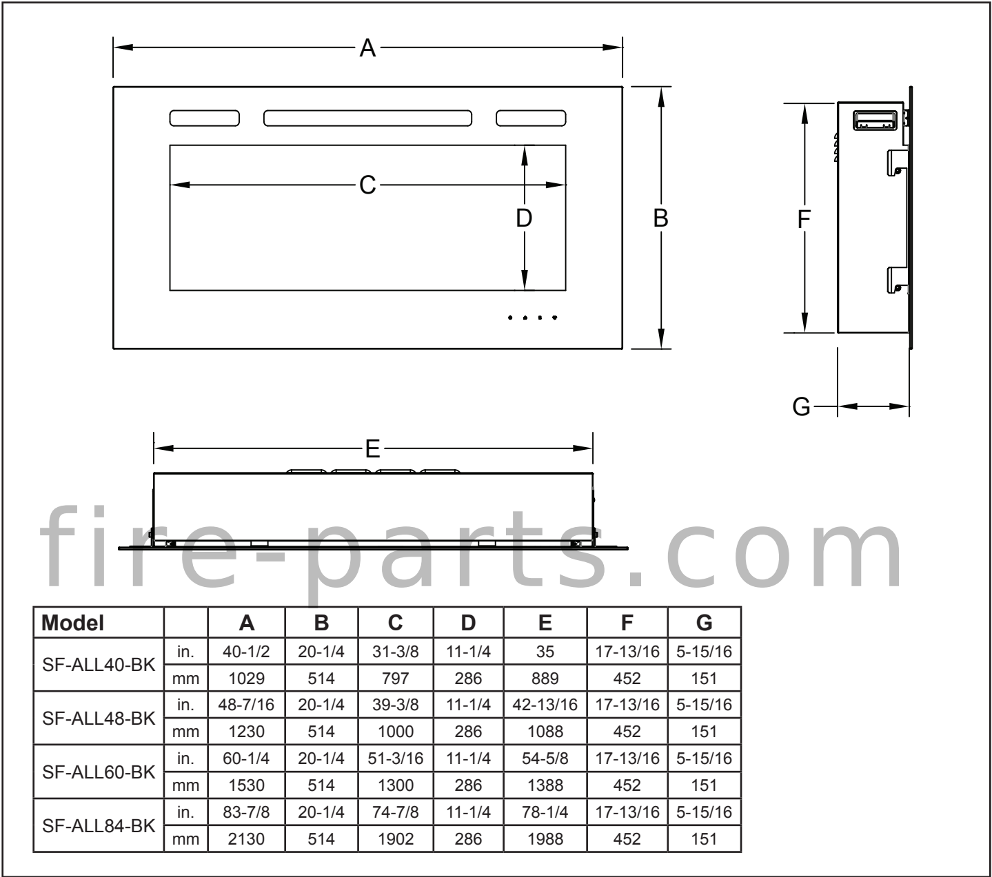
Figure 3.1 Appliance Dimensions
