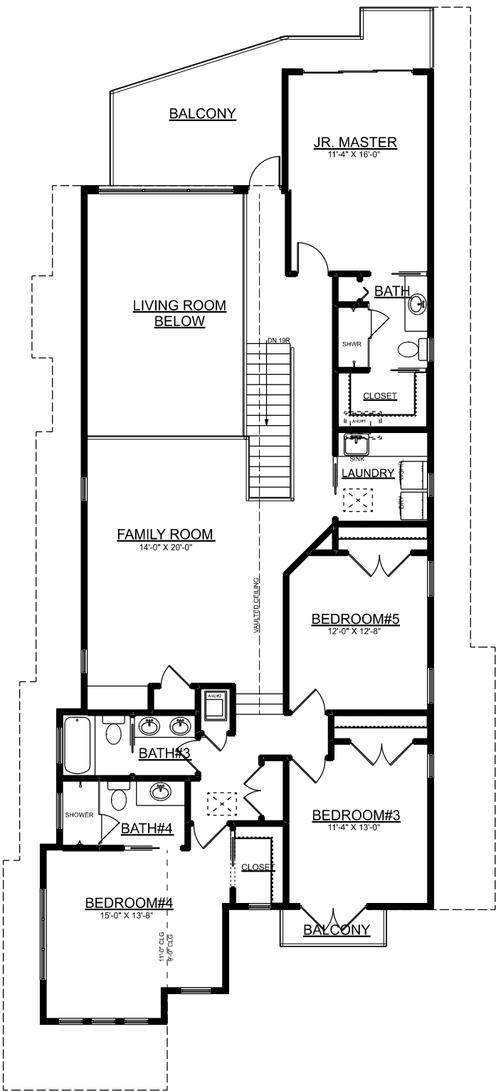
LOT 6 SECOND FLOOR PLAN
