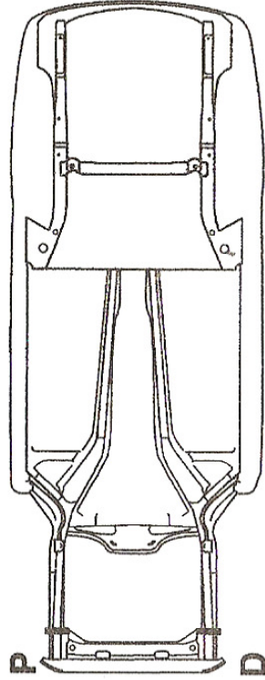
UNDERBODY VIEW
