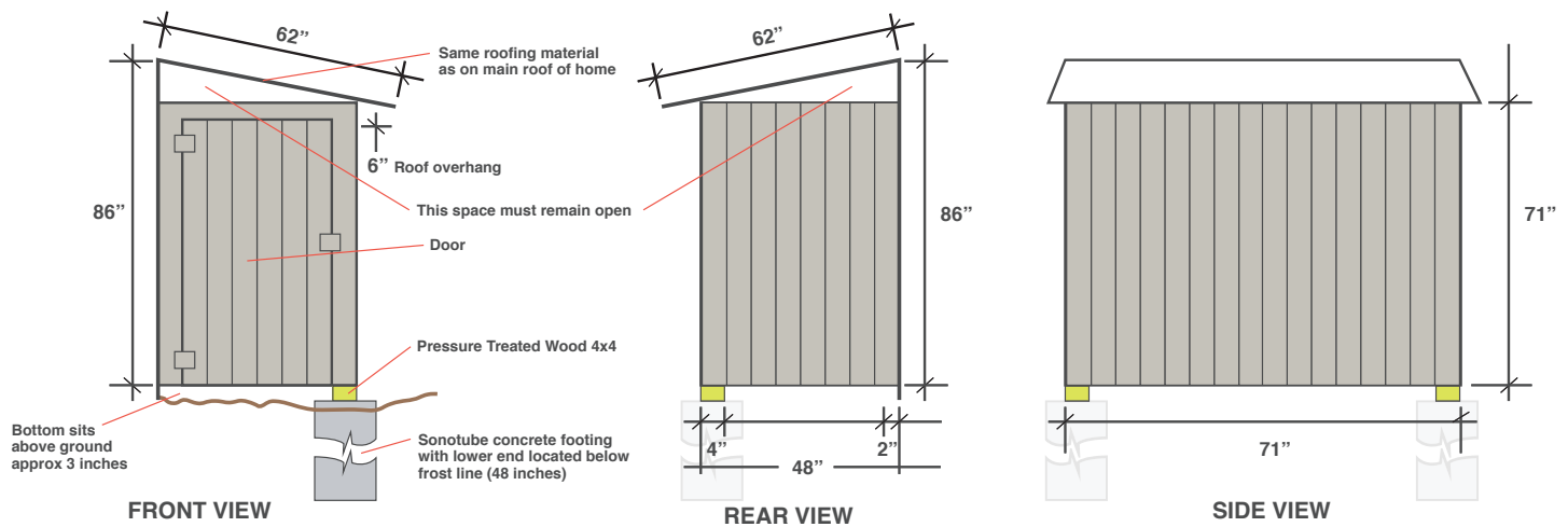
Figure 2. Propane Shed
