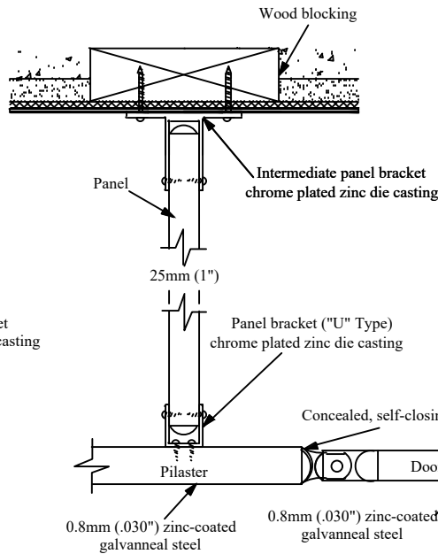
plan detail A-A
