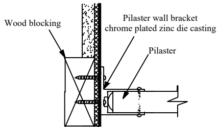
plan detail D-D
