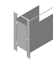
Floor Mounted Overhead Braced
