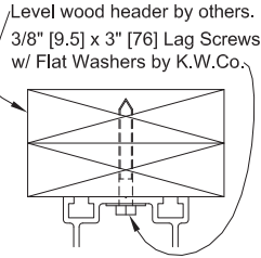
Optional Direct Mount
