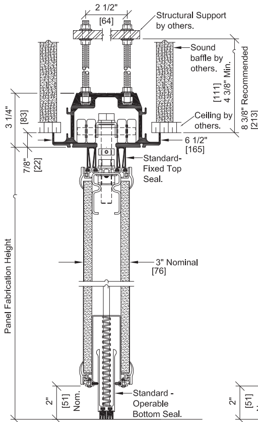
850 Hinged Pairs Aluminum Track and Carrier
