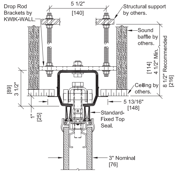
850 Hinged Pairs Steel Track and Carrier
