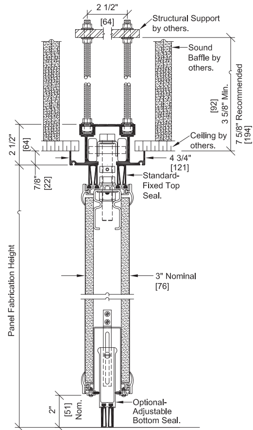
425 Hinged Pairs Aluminum Track and Carrier
