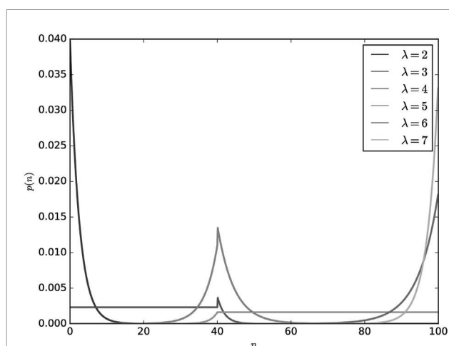
FIGURE 4 Influence of \lambda on the probability of having n energy packets in the battery for \mu_1 = 3 , \mu_2 = 5 , B = 100 , and K = 40 .
