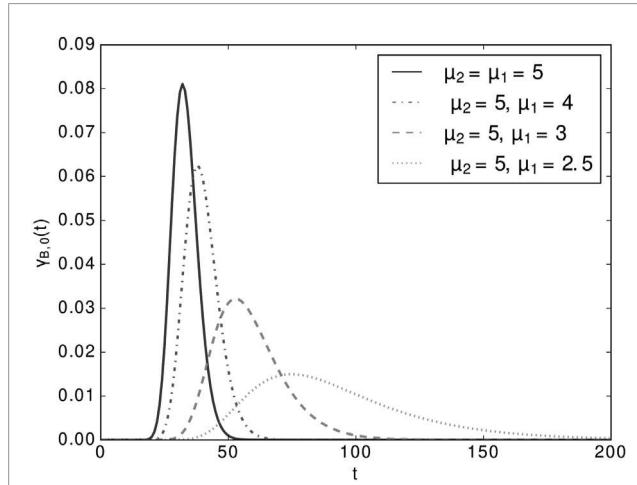
FIGURE 6 Influence of \mu_1 on the density of the lifetime of the IoT node y_{B,0}(t) for \mu_2 = 5 , \lambda = 2 , B = 100 , and K = 40 .
