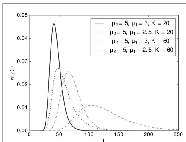
FIGURE 5 Influence of the proposed energy-saving threshold policy on the density of the lifetime of the IoT node y_{B,0}(t) for K = 20, 60 , \mu_2 = 5 , \lambda = 2 , and B = 100 .
