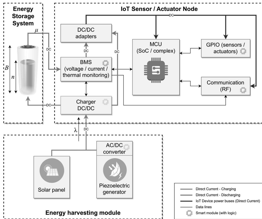
FIGURE 1 Architecture of a self-powered green IoT sensor node.
