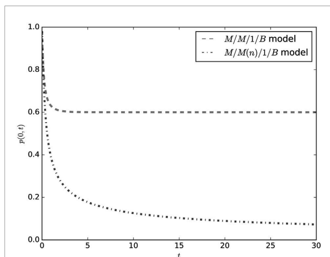
FIGURE 3 Comparison of the transient probability of service outage p(0,t) from the M/M/1/B and M/M(n)/1/B for \mu_1 = 2 , \mu_2 = 5 , \lambda = 2 , K = 40 , and B = 100 .
