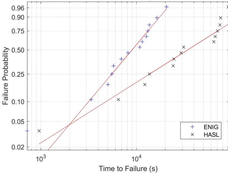
Figure 22. Weibull plots for Pb HASL and ENIG whole PCB/board vibration failures (Blue plus sign =ENIG, black cross symbol = Pb HASL) Weibull probability plot from vibration testing results, with two linear distributions for flip chips on Pb HASL finished PCBs (black cross markers) and ENIG finished PCBs (blue plus marker). The x-axis represents the time to failure in seconds in logarithmic scale. The y-axis represents the Weibull failure probability ranging from 0 to 1 in logarithmic scale. Pb HASL reliability reaches about 90,000 seconds, with a slope of 0.765. ENIG reliability reaches about 20,000 seconds, with a slope of 1.297.
