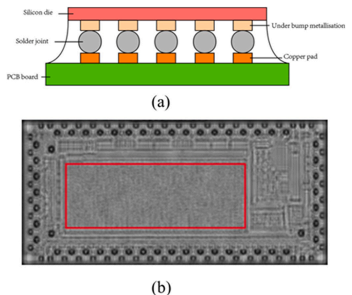
Fig. 7. (a)Cross-section schematic of a typical flip-chip on board assembly; (b) An ultrasonic C-scan image of the silicon die to solder joint interface of the flip-chip assembly. (For interpretation of the references to colour in this figure legend, the reader is referred to the Web version of this article.)
