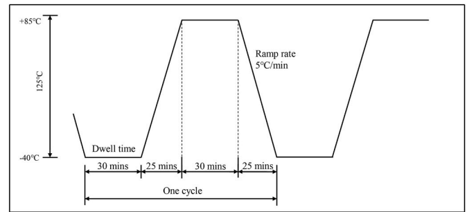
Fig. 6. The thermal profile used in the accelerated thermal cycling test.
