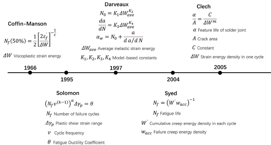
Fig. 1. Electronic packaging fatigue life prediction model and its evolution [8–10].
