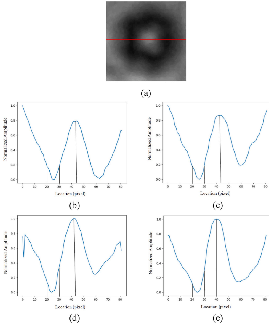
Fig. 14. (a) A solder joint image; the C-line plots along the red line from the solder joint images of (b) 0 cycle, (c) 100 cycle, (d) 200 cycle, and (e) 352 cycle. (For interpretation of the references to colour in this figure legend, the reader is referred to the Web version of this article.)
