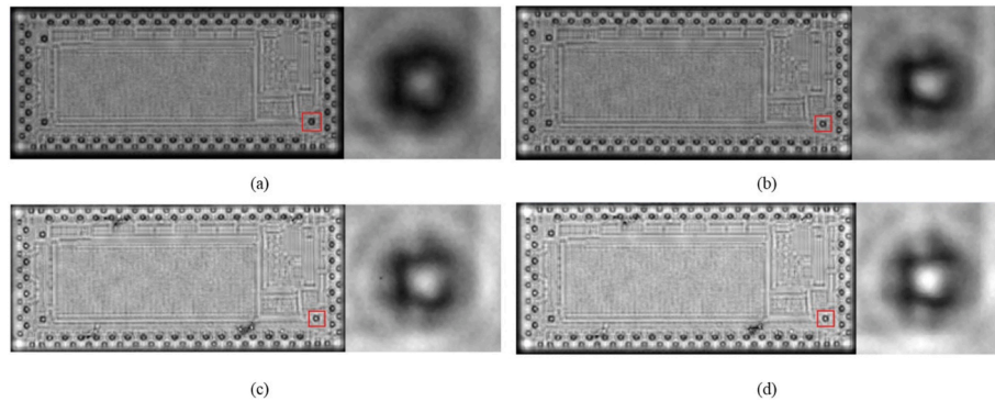
Fig. 8. Ultrasonic images of a flip-chip package obtained after (a) 0 cycles ATC test; (b) 100 cycles; (c) 200 cycles; (d) 352 cycles. The enlarged images in the right side is from the solder joints marked in red in the left side images. (For interpretation of the references to colour in this figure legend, the reader is referred to the Web version of this article.)
