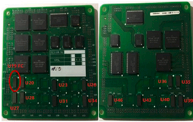
Fig. 4. Flip-chip packages on the front and back side of test board.
