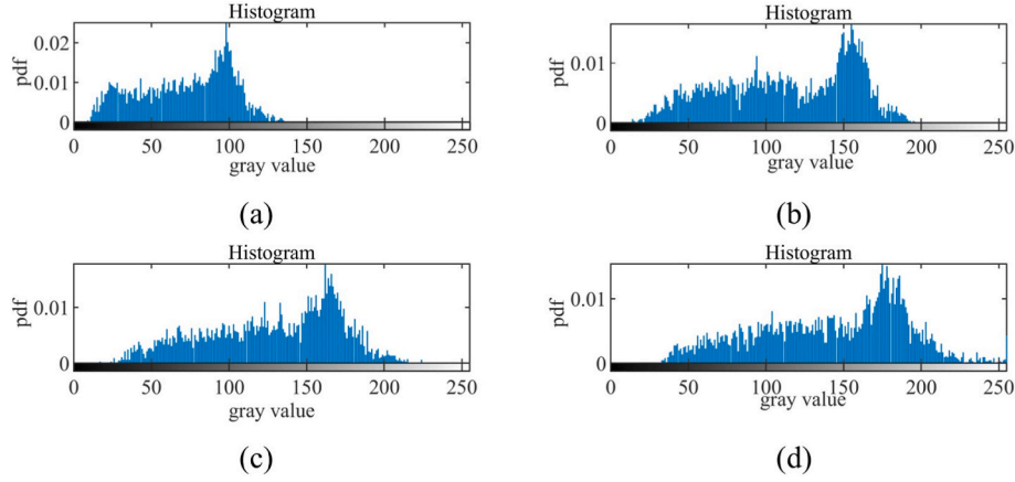
Fig. 10. Grayscale distribution of solder joints in diverse cycles: (a) 100 cycle, (b) 104 cycle, (c) 108 cycle, (d) 112 cycle. Pdf: probability density function.
