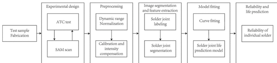
Fig. 2. Flowchart of the proposed methodology.
