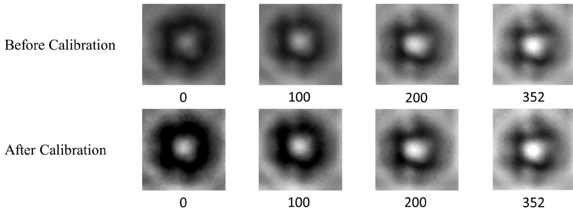
Fig. 11. Solder joint images at 0,100,200,352 cycles before and after intensity calibration.
