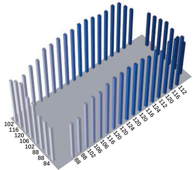
Fig. 20. Reliability of individual solder joints.
