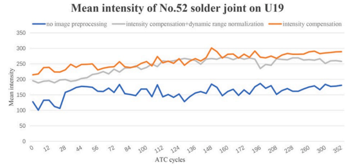
Fig. 17. ROI mean intensity versus ATC test cycles.
