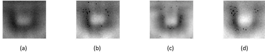
Fig. 9. The ultrasonic image of solder joint No.6 on flip-chip U19 after (a) 0, (b) 100, (c) 200, (d) 352 cycles.
