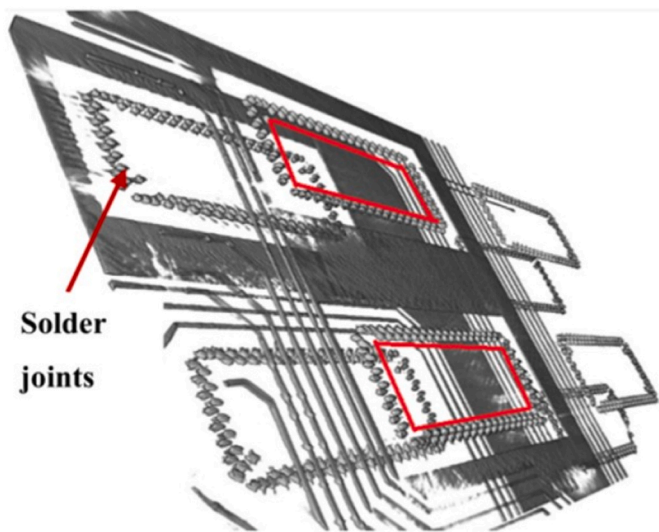
Fig. 5. 3D X-ray image of flip-chip structure Schematic shows the layout of flip-chip packages in the PCB board.
