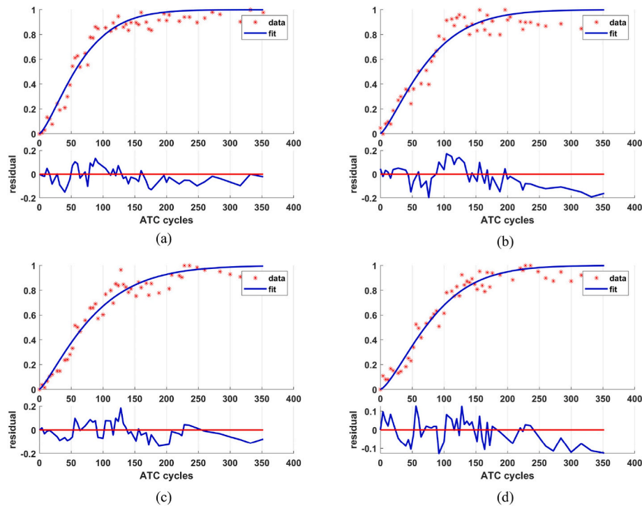
Fig. 19. Failure model of solder joint (a)No.40, (b)No.42, (c)No.44, (d)No.46.
