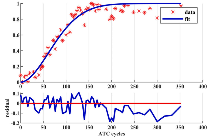
Fig. 18. Establishment of the failure model by curve fitting.
