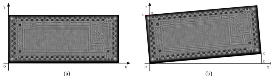
Fig. 13. Ultrasonic image level alignment. (a) A perfectly aligned ultrasonic image; (b) a tilted flip-chip image.
