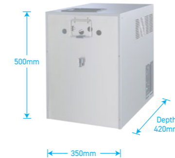
65L Underbench Unit
