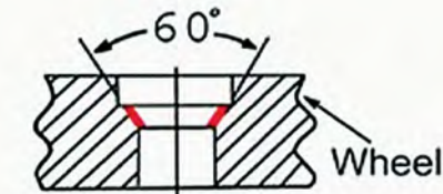
Acorn/Tapered Seat
