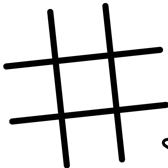
tic-tac-toe
