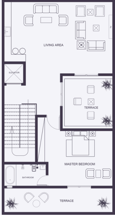
الملحق Second Floor
