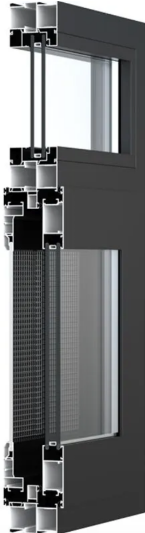
128 Series Aluminium Casement Window Double Thermal Break with Integrated Screen
