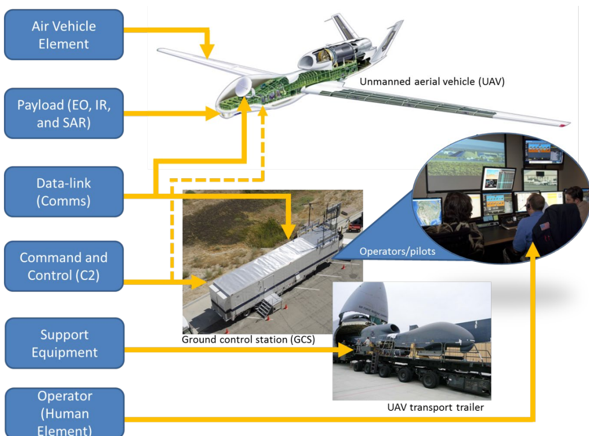
Figure 1. Basic UAS configuration with major elements identified.
