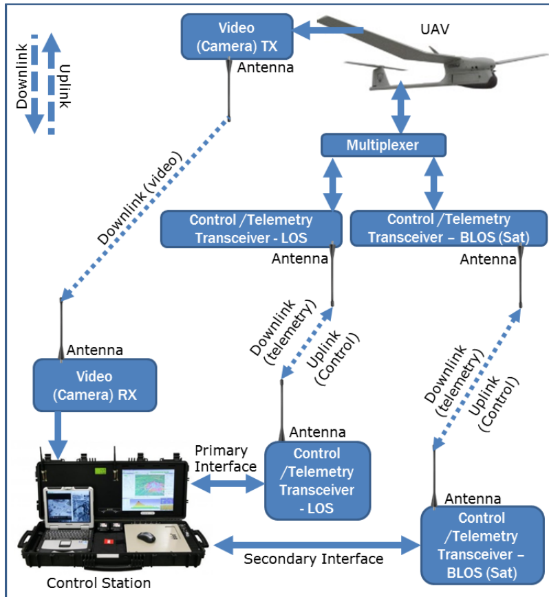
Figure 3. Example C3 configuration and associated interfaces.
