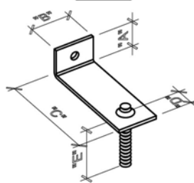
"L" STRAP W/ WELDED ALL THREAD PIN ISOMETRIC
