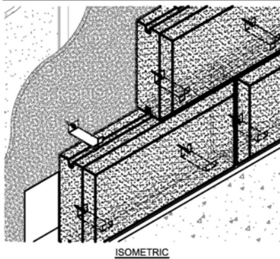
DETAIL 4-"SPLIT TAIL" STRAP @ VENEER
