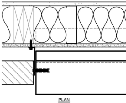
DETAIL 4-"SPLIT TAIL" STRAP @ VENEER
