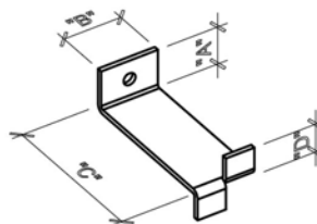
"SPLIT TAIL" STRAP ISOMETRIC
