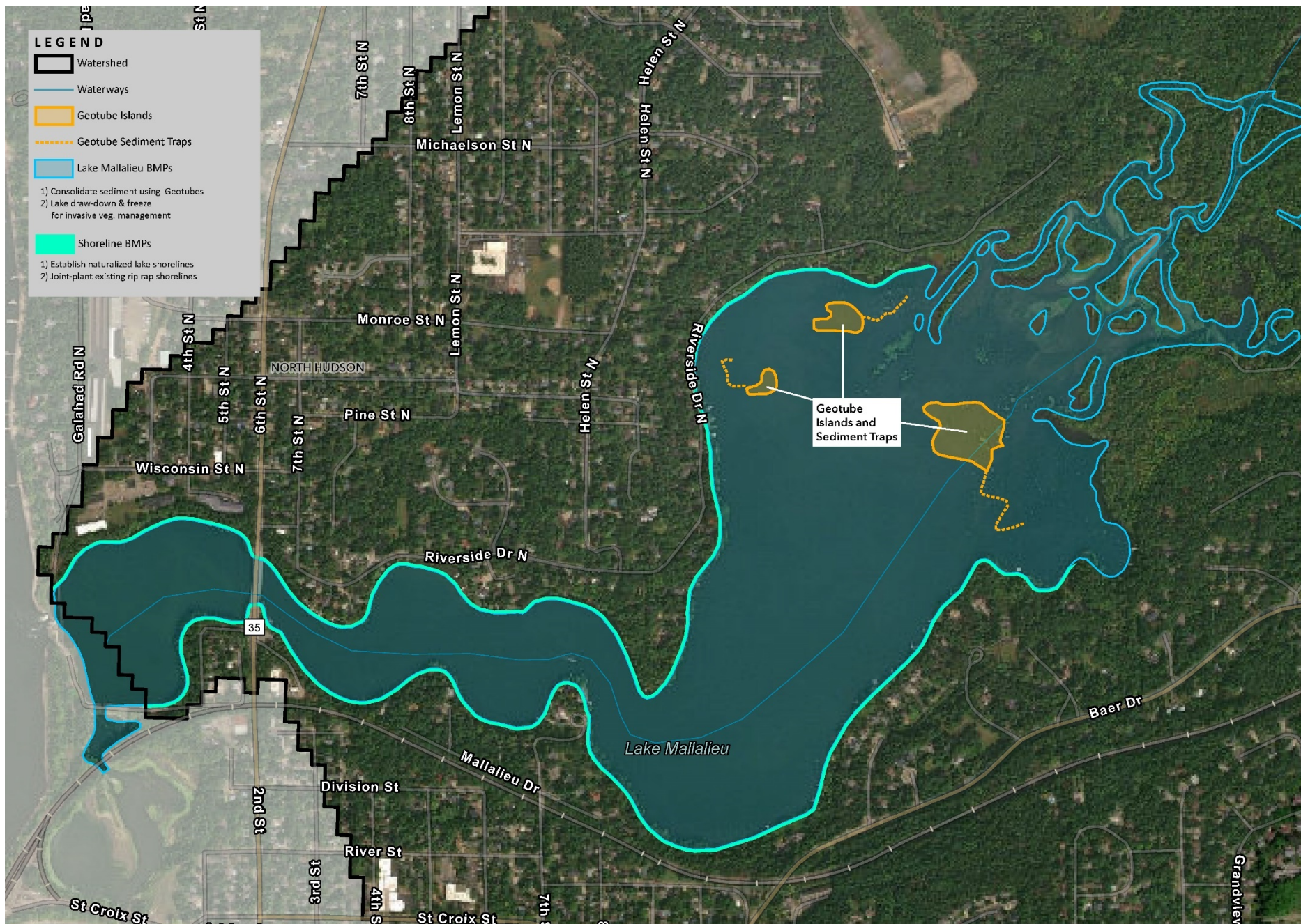
EXHIBIT 7: POTENTIAL LOCATIONS FOR LAKE MALLALIEU SHORELINE AND IN-LAKE BMPs
