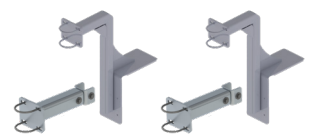
RAISED PIPE MOUNT TO FIXED DOCK KIT 302081 FOR 2-3" PIPE 302082 FOR 4" PIPE EXTRA SUPPORT AVAILABLE
