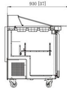
TSSU-40MT
