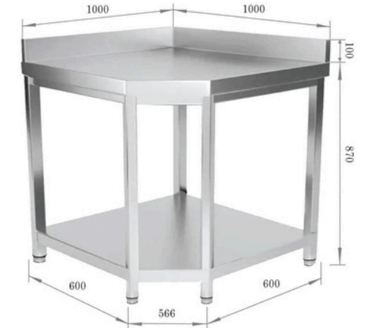
Work table with backsplash
