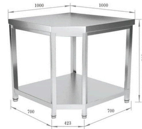
Work table without backsplash
