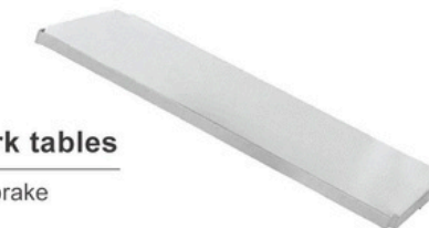
Intermediate shelf for work table • Width: 600mm and 700mm • Length from 600mm to 2000mm
