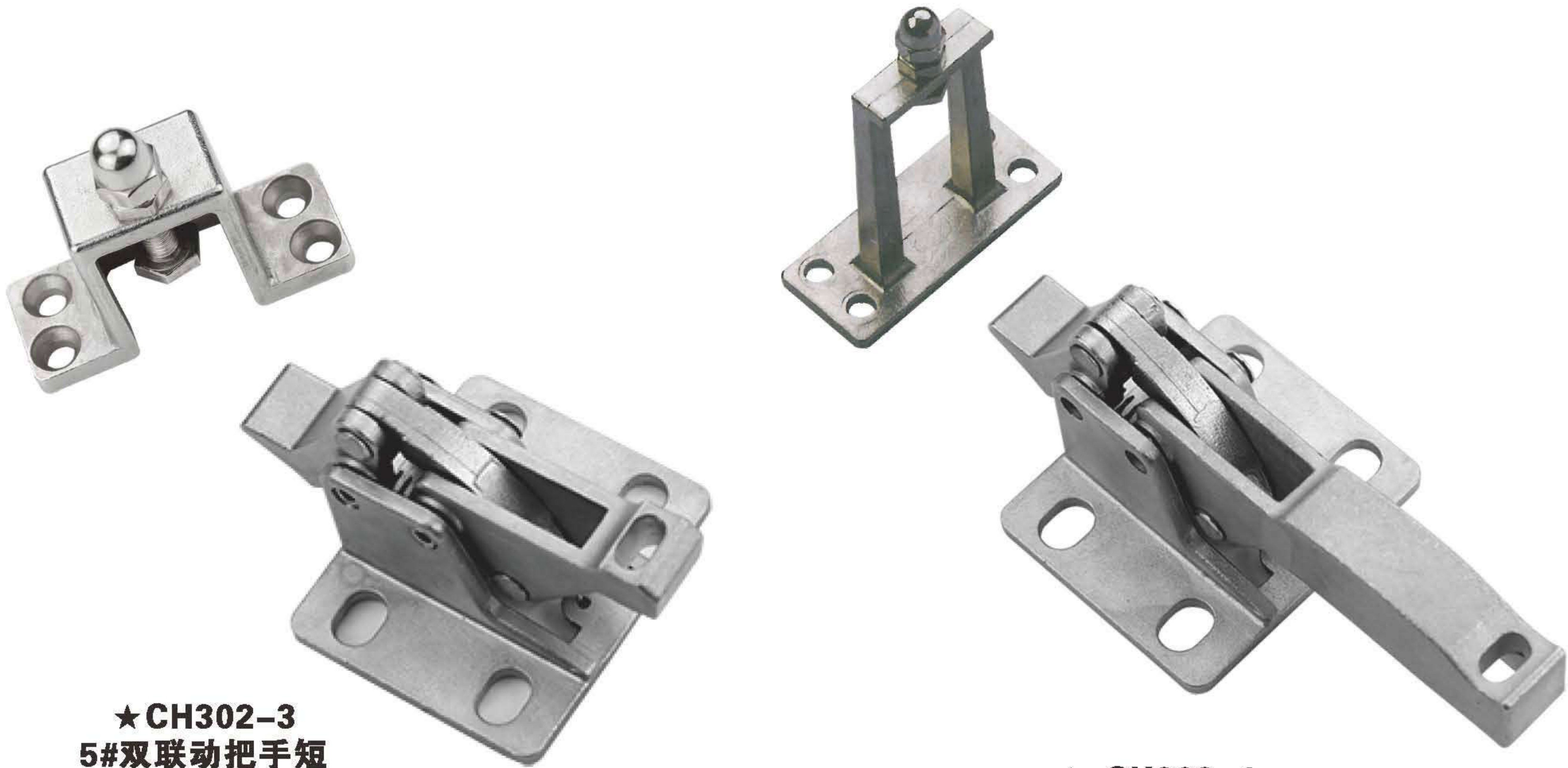
★ CH302-4 5#双联动把手长
