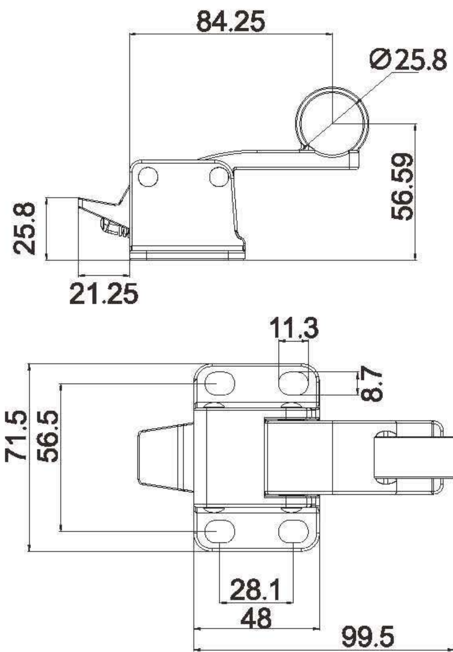
B款方底双联动把手 CH302-9
