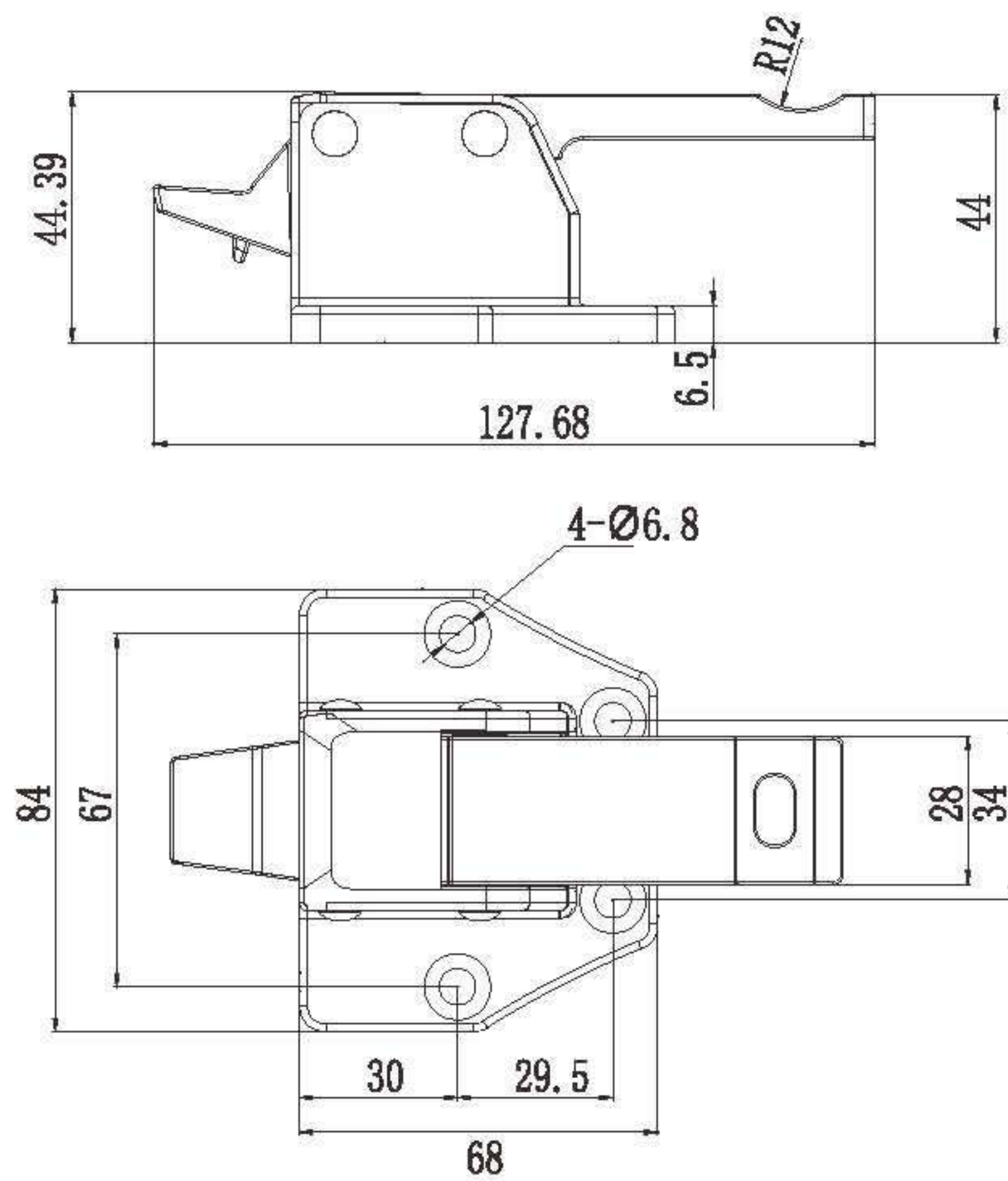
CH302-16 A4款双联动把手焊接型
