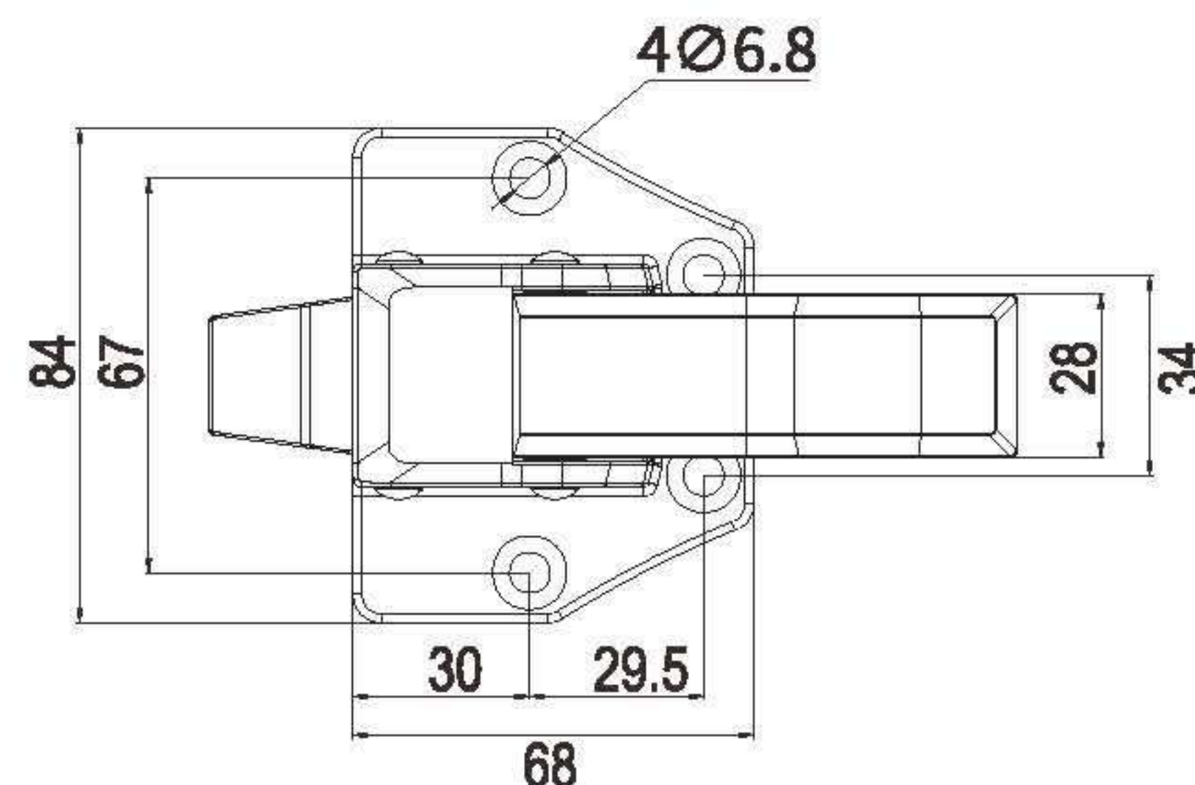
A4款双联动把手 CH302-15
