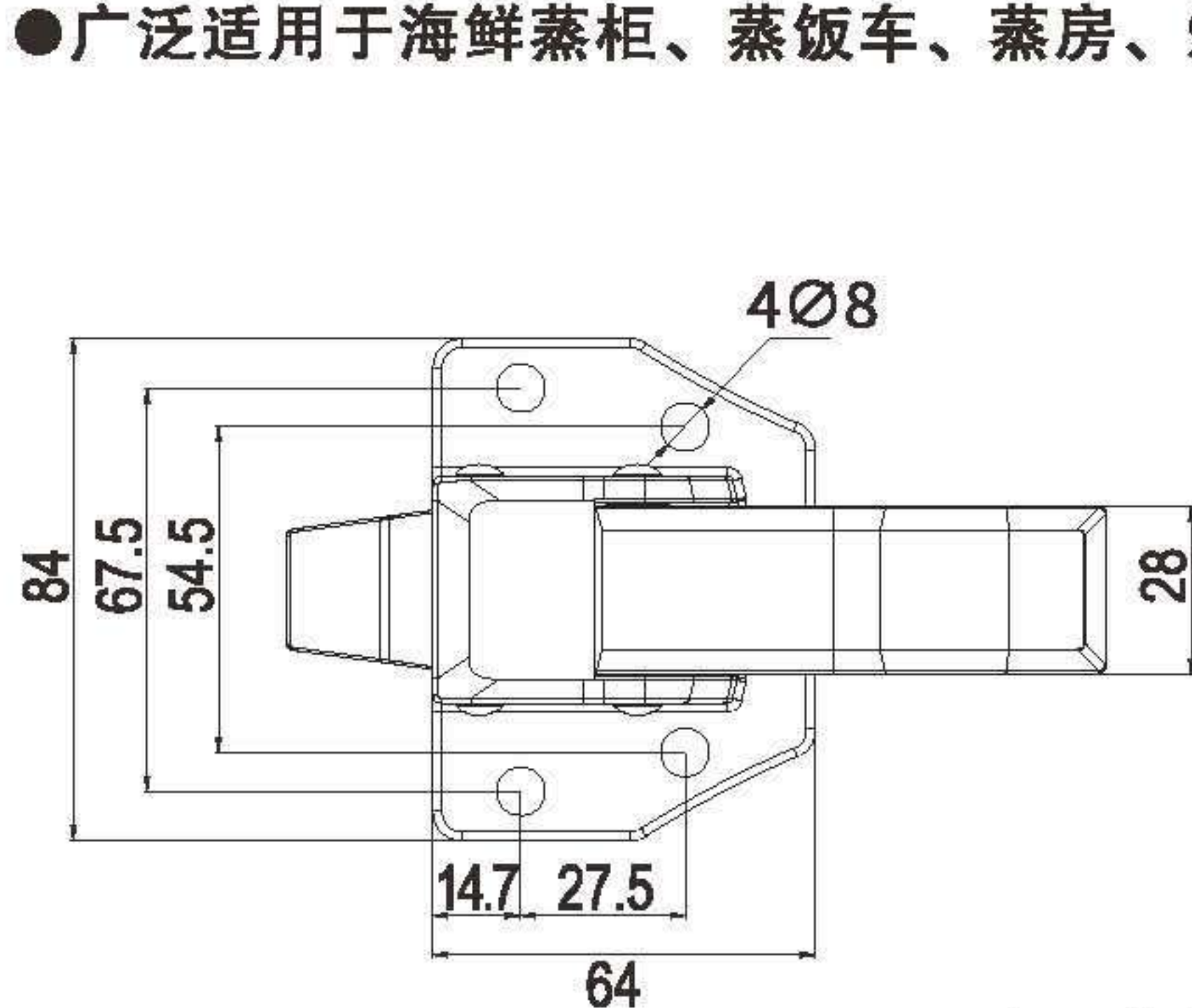
A3款双联动把手 CH302-13
