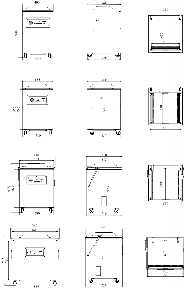
DZQ-400/500/600/800 Vertical Vacuum Packing Machine 立式真空包装机
