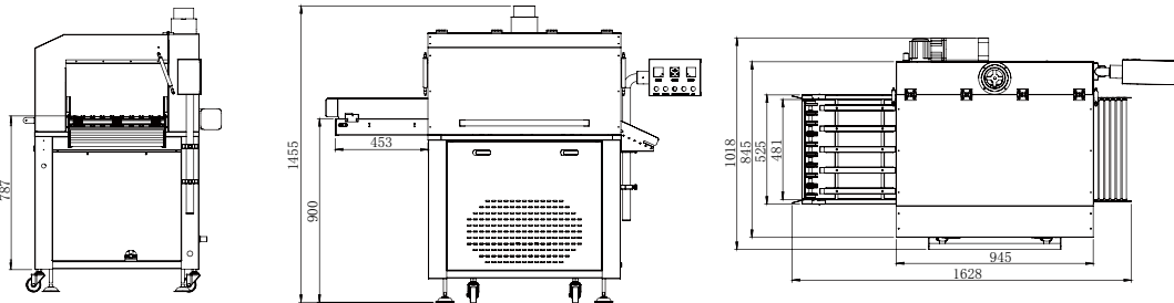
ST-8031/10065 Hot Water Shrink Tunnel 隧道式热水收缩机
