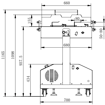
DZQ-600 2SAT Double chamber Vacuum Packing Machine 翻转式双室真空包装机
