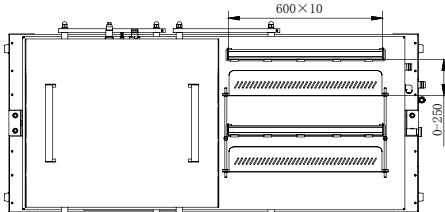
DZQ-600 2SAT Double chamber Vacuum Packing Machine 翻转式双室真空包装机
