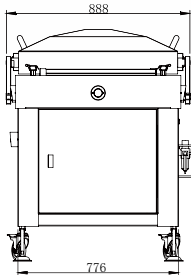
DZQ-850 2SE Double chamber Vacuum Packing Machine 双室真空包装机
