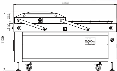
DZQ-850 2SE Double chamber Vacuum Packing Machine 双室真空包装机
