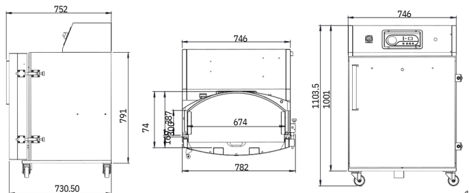
DZL-600 Vertical Chamber Vacuum Packing Machine 立式真空包装机
